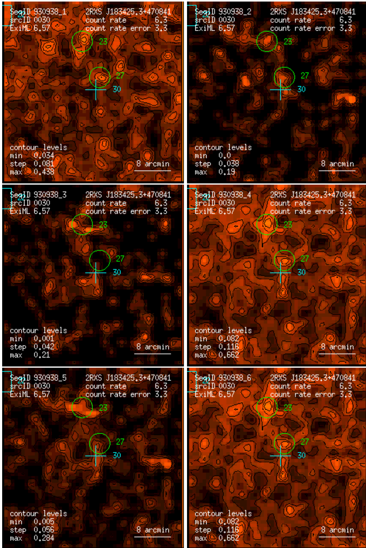
Figure 30: RASS 930938: detection 0030: band rate images, Gaussian filter: (1) PSPC channels 11 – 41, (2) 52 – 90, (3) 91 – 201, (4) 11 – 235, (5) 52 – 201, (6) 11 – 201. Broad band rates in counts/ks. Band rate contour levels in counts/ks/arcmin 2 .
