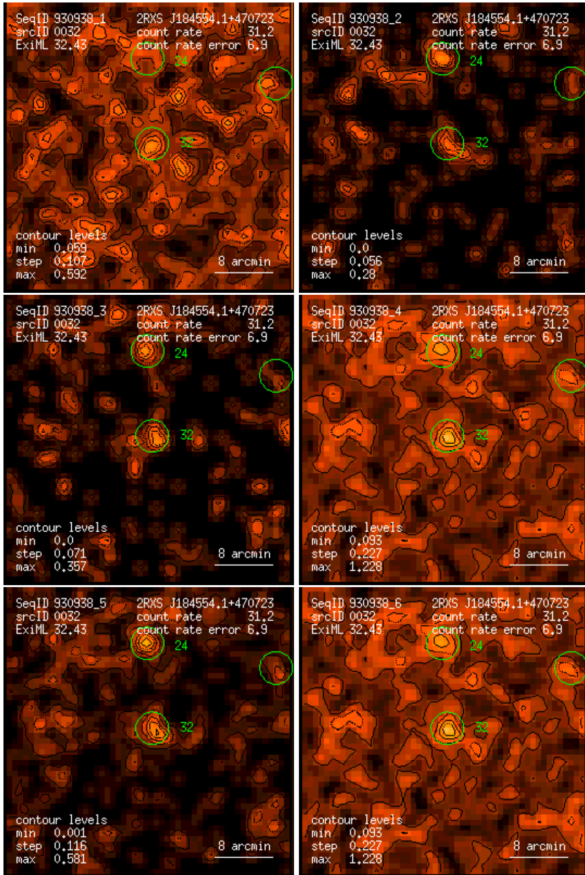
Figure 32: RASS 930938: detection 0032: band rate images, Gaussian filter: (1) PSPC channels 11 – 41, (2) 52 – 90, (3) 91 – 201, (4) 11 – 235, (5) 52 – 201, (6) 11 – 201. Broad band rates in counts/ks. Band rate contour levels in counts/ks/arcmin 2 .
