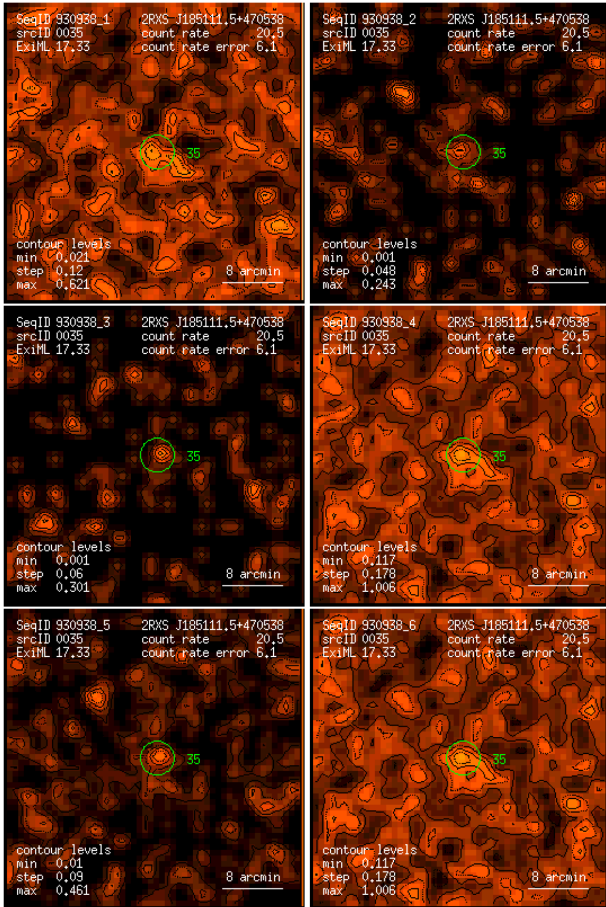
Figure 35: RASS 930938: detection 0035: band rate images, Gaussian filter: (1) PSPC channels 11 – 41, (2) 52 – 90, (3) 91 – 201, (4) 11 – 235, (5) 52 – 201, (6) 11 – 201. Broad band rates in counts/ks. Band rate contour levels in counts/ks/arcmin 2 .
