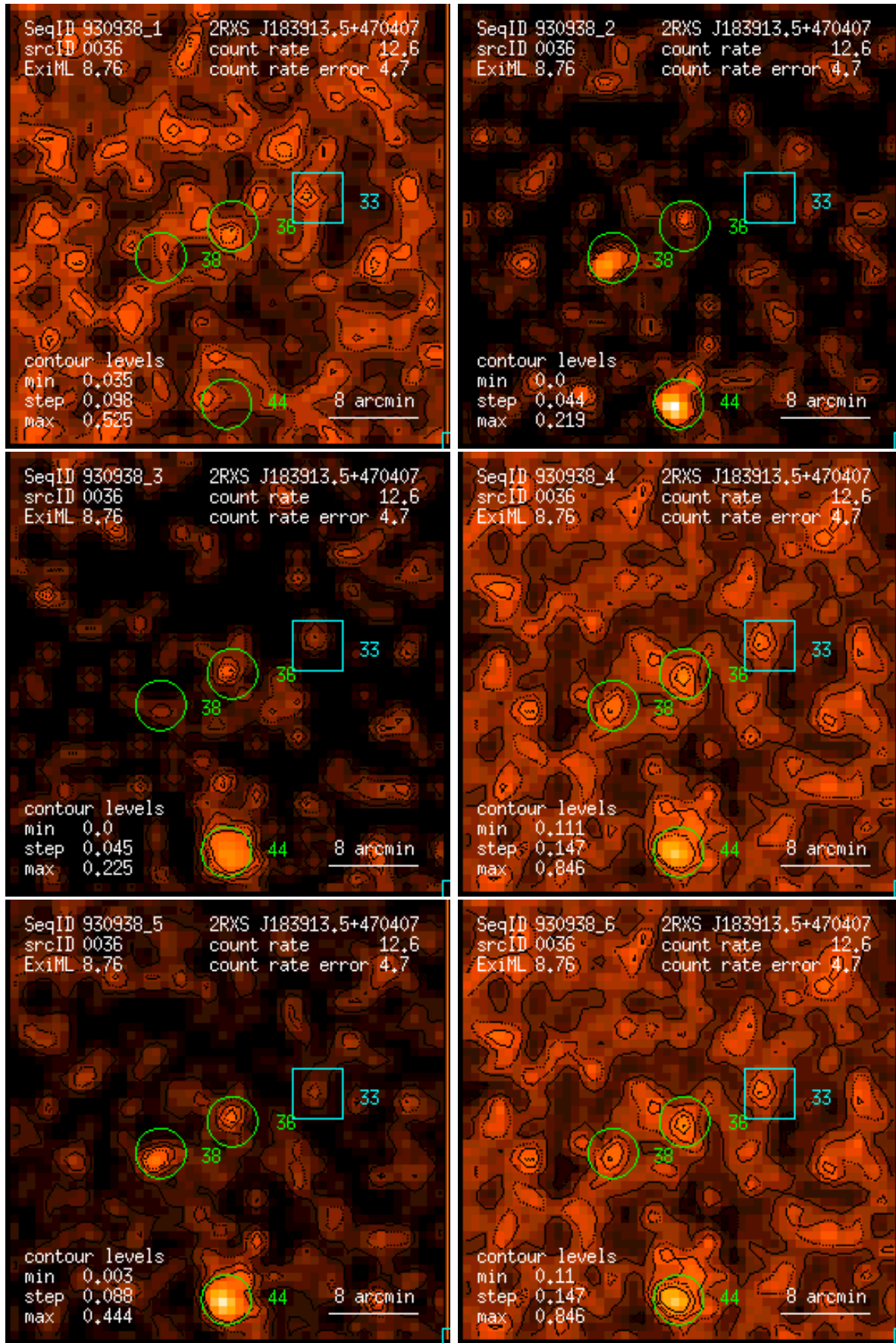
Figure 36: RASS 930938: detection 0036: band rate images, Gaussian filter: (1) PSPC channels 11 – 41, (2) 52 – 90, (3) 91 – 201, (4) 11 – 235, (5) 52 – 201, (6) 11 – 201. Broad band rates in counts/ks. Band rate contour levels in counts/ks/arcmin 2 .
