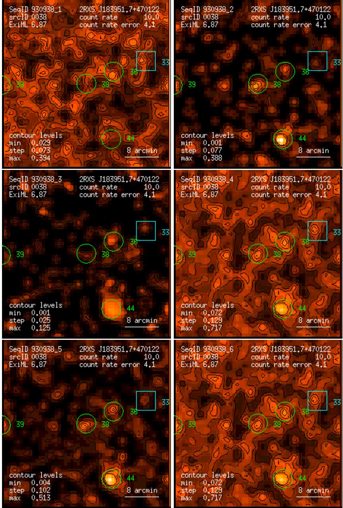
Figure 38: RASS 930938: detection 0038: band rate images, Gaussian filter: (1) PSPC channels 11 – 41, (2) 52 – 90, (3) 91 – 201, (4) 11 – 235, (5) 52 – 201, (6) 11 – 201. Broad band rates in counts/ks. Band rate contour levels in counts/ks/arcmin 2 .
