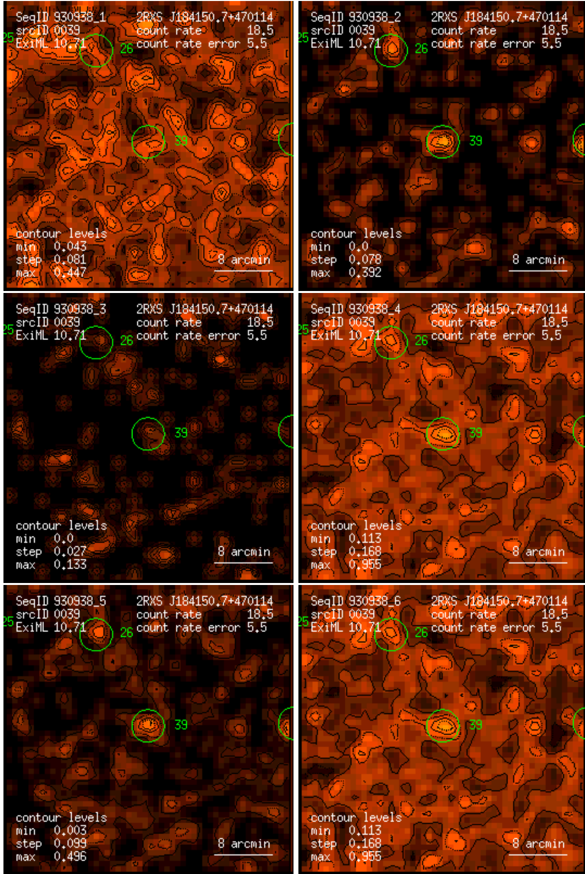
Figure 39: RASS 930938: detection 0039: band rate images, Gaussian filter: (1) PSPC channels 11 – 41, (2) 52 – 90, (3) 91 – 201, (4) 11 – 235, (5) 52 – 201, (6) 11 – 201. Broad band rates in counts/ks. Band rate contour levels in counts/ks/arcmin 2 .
