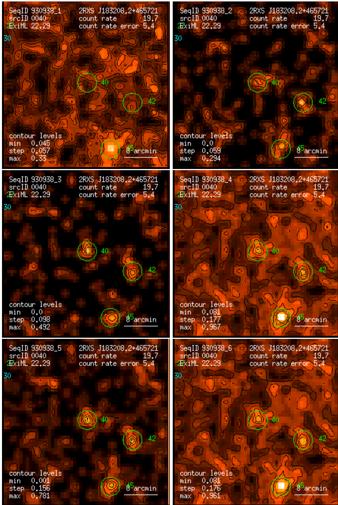
Figure 40: RASS 930938: detection 0040: band rate images, Gaussian filter: (1) PSPC channels 11 – 41, (2) 52 – 90, (3) 91 – 201, (4) 11 – 235, (5) 52 – 201, (6) 11 – 201. Broad band rates in counts/ks. Band rate contour levels in counts/ks/arcmin 2 .
