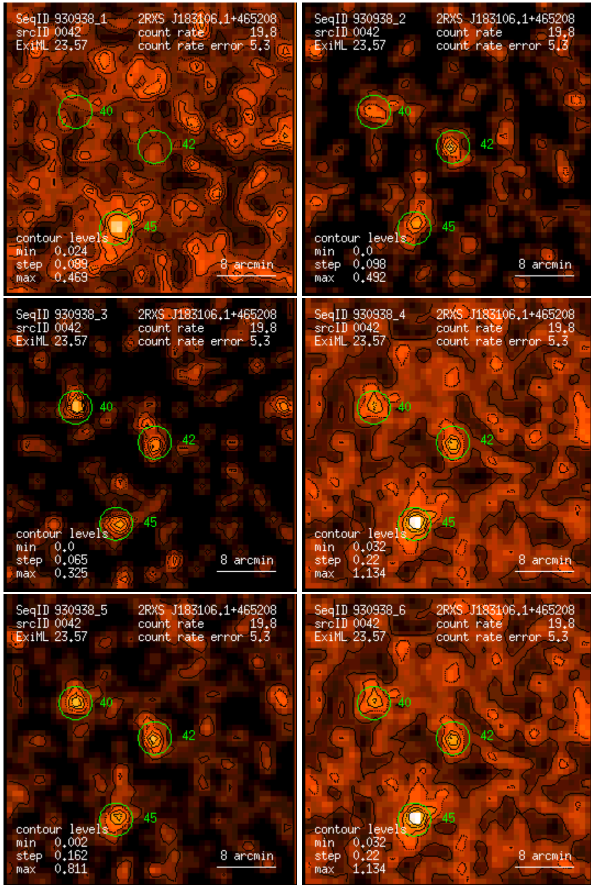
Figure 42: RASS 930938: detection 0042: band rate images, Gaussian filter: (1) PSPC channels 11 – 41, (2) 52 – 90, (3) 91 – 201, (4) 11 – 235, (5) 52 – 201, (6) 11 – 201. Broad band rates in counts/ks. Band rate contour levels in counts/ks/arcmin 2 .
