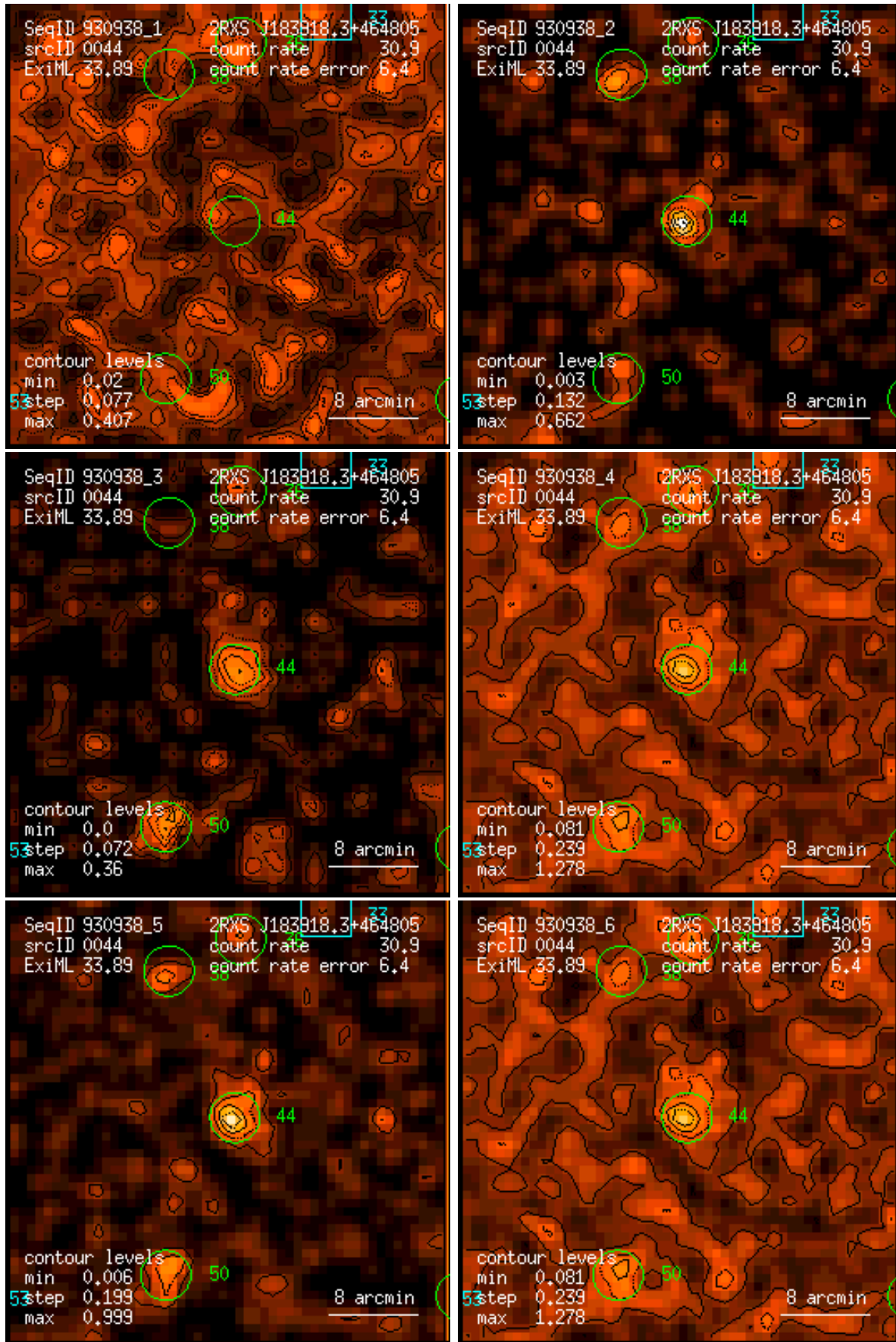
Figure 44: RASS 930938: detection 0044: band rate images, Gaussian filter: (1) PSPC channels 11 – 41, (2) 52 – 90, (3) 91 – 201, (4) 11 – 235, (5) 52 – 201, (6) 11 – 201. Broad band rates in counts/ks. Band rate contour levels in counts/ks/arcmin 2 .
