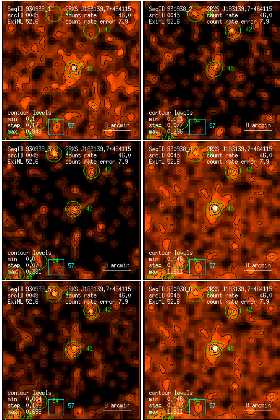
Figure 45: RASS 930938: detection 0045: band rate images, Gaussian filter: (1) PSPC channels 11 – 41, (2) 52 – 90, (3) 91 – 201, (4) 11 – 235, (5) 52 – 201, (6) 11 – 201. Broad band rates in counts/ks. Band rate contour levels in counts/ks/arcmin 2 .
