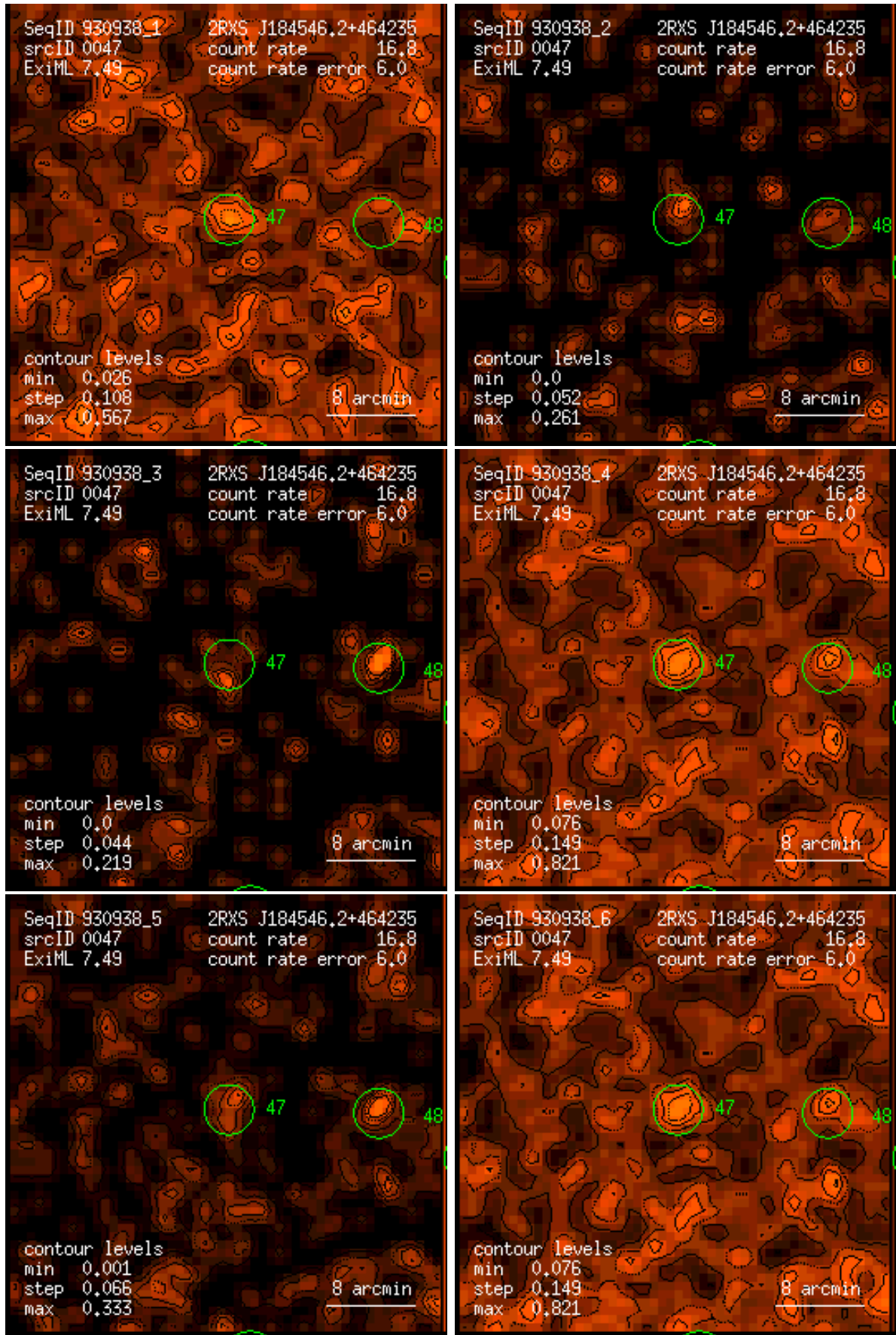
Figure 47: RASS 930938: detection 0047: band rate images, Gaussian filter: (1) PSPC channels 11 – 41, (2) 52 – 90, (3) 91 – 201, (4) 11 – 235, (5) 52 – 201, (6) 11 – 201. Broad band rates in counts/ks. Band rate contour levels in counts/ks/arcmin 2 .
