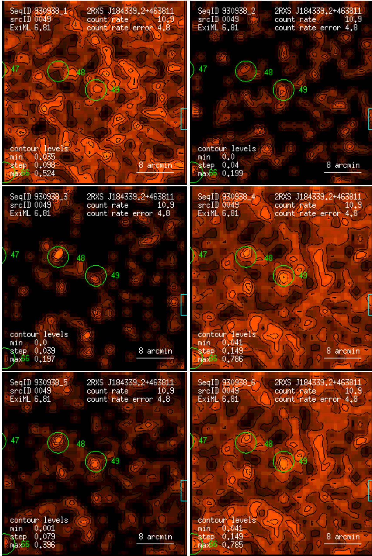
Figure 49: RASS 930938: detection 0049: band rate images, Gaussian filter: (1) PSPC channels 11 – 41, (2) 52 – 90, (3) 91 – 201, (4) 11 – 235, (5) 52 – 201, (6) 11 – 201. Broad band rates in counts/ks. Band rate contour levels in counts/ks/arcmin 2 .
