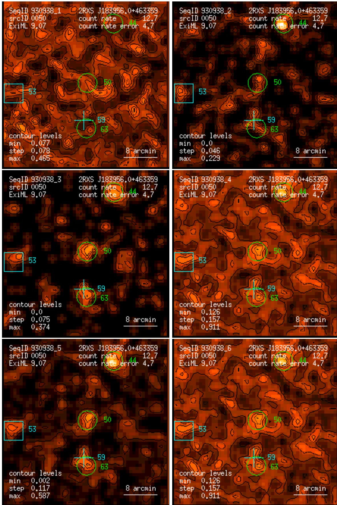
Figure 50: RASS 930938: detection 0050: band rate images, Gaussian filter: (1) PSPC channels 11 – 41, (2) 52 – 90, (3) 91 – 201, (4) 11 – 235, (5) 52 – 201, (6) 11 – 201. Broad band rates in counts/ks. Band rate contour levels in counts/ks/arcmin 2 .
