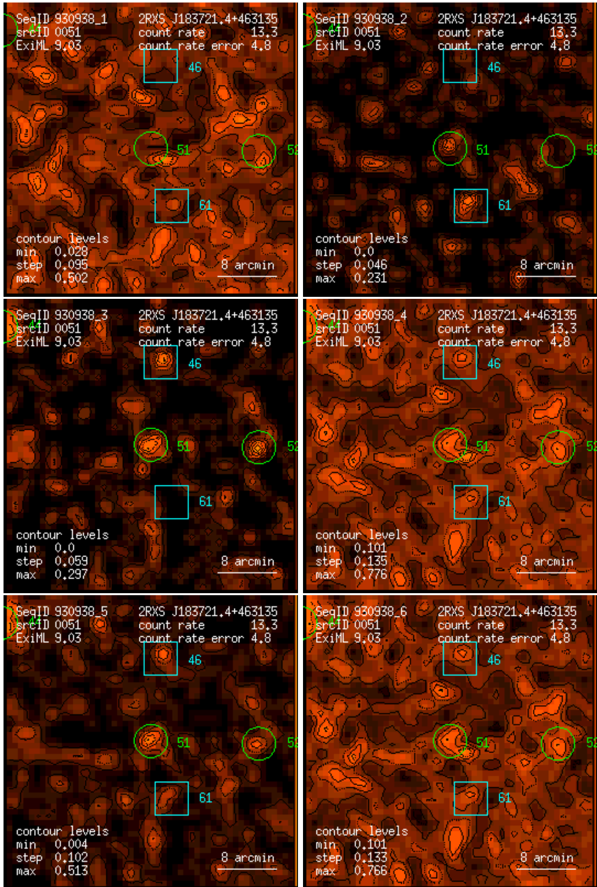
Figure 51: RASS 930938: detection 0051: band rate images, Gaussian filter: (1) PSPC channels 11 – 41, (2) 52 – 90, (3) 91 – 201, (4) 11 – 235, (5) 52 – 201, (6) 11 – 201. Broad band rates in counts/ks. Band rate contour levels in counts/ks/arcmin 2 .
