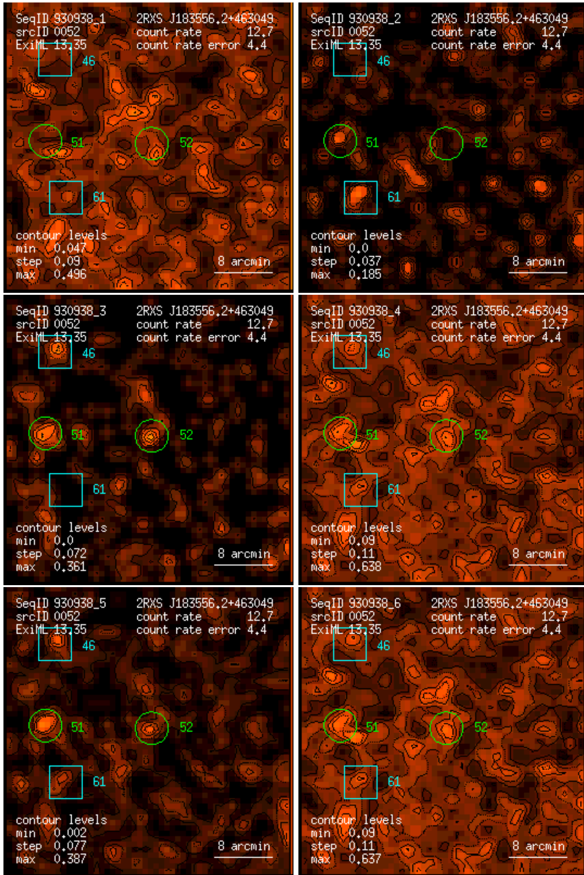
Figure 52: RASS 930938: detection 0052: band rate images, Gaussian filter: (1) PSPC channels 11 – 41, (2) 52 – 90, (3) 91 – 201, (4) 11 – 235, (5) 52 – 201, (6) 11 – 201. Broad band rates in counts/ks. Band rate contour levels in counts/ks/arcmin 2 .
