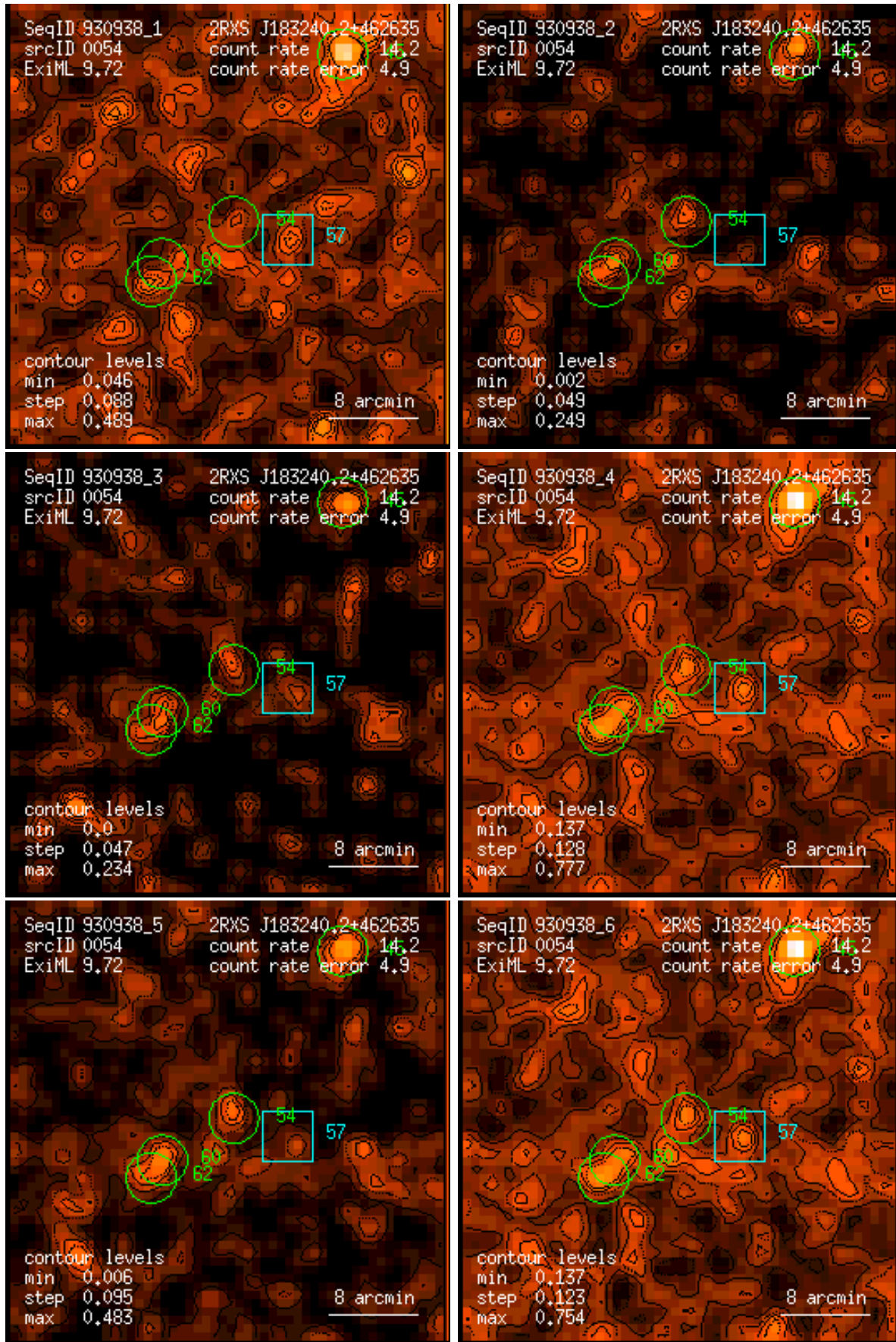
Figure 54: RASS 930938: detection 0054: band rate images, Gaussian filter: (1) PSPC channels 11 – 41, (2) 52 – 90, (3) 91 – 201, (4) 11 – 235, (5) 52 – 201, (6) 11 – 201. Broad band rates in counts/ks. Band rate contour levels in counts/ks/arcmin 2 .
