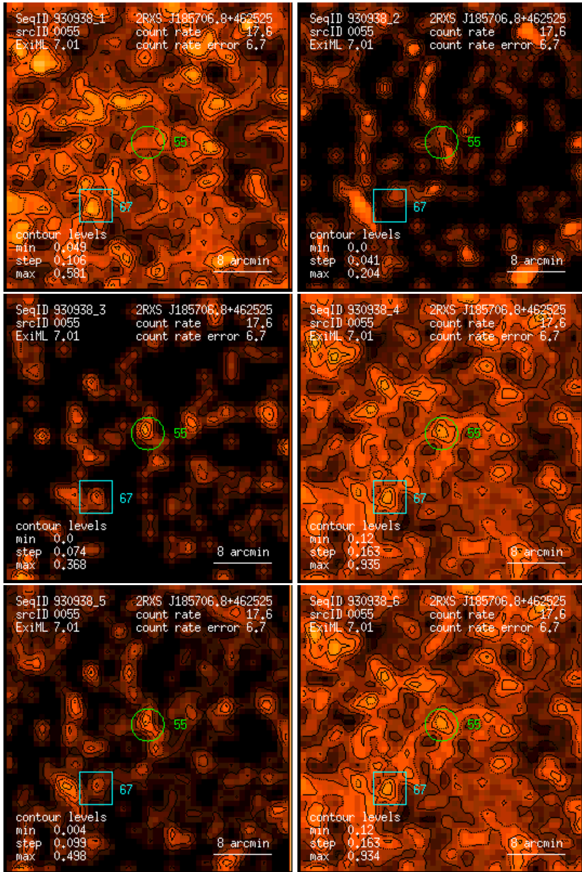
Figure 55: RASS 930938: detection 0055: band rate images, Gaussian filter: (1) PSPC channels 11 – 41, (2) 52 – 90, (3) 91 – 201, (4) 11 – 235, (5) 52 – 201, (6) 11 – 201. Broad band rates in counts/ks. Band rate contour levels in counts/ks/arcmin 2 .
