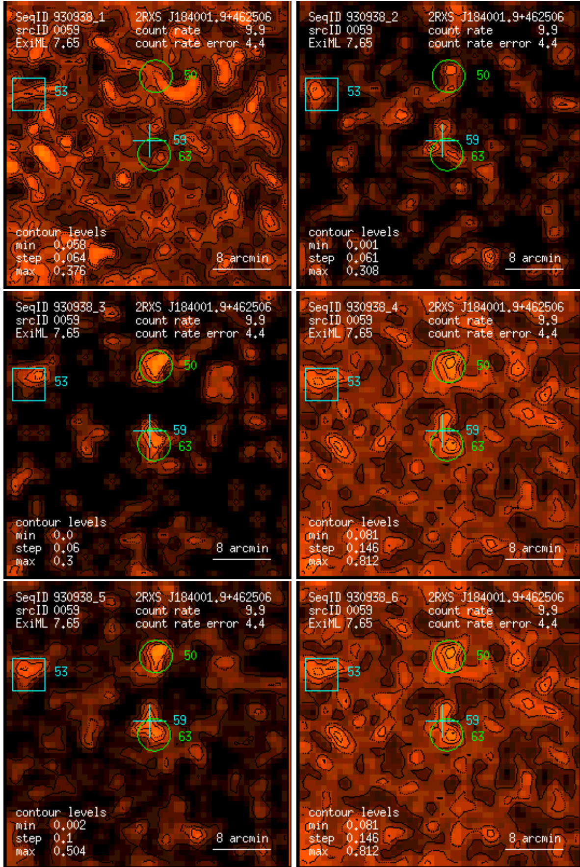
Figure 59: RASS 930938: detection 0059: band rate images, Gaussian filter: (1) PSPC channels 11 – 41, (2) 52 – 90, (3) 91 – 201, (4) 11 – 235, (5) 52 – 201, (6) 11 – 201. Broad band rates in counts/ks. Band rate contour levels in counts/ks/arcmin 2 .
