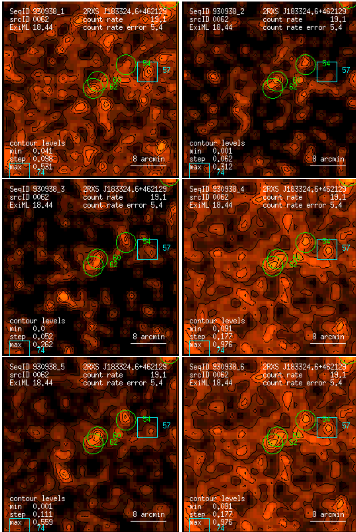
Figure 62: RASS 930938: detection 0062: band rate images, Gaussian filter: (1) PSPC channels 11 – 41, (2) 52 – 90, (3) 91 – 201, (4) 11 – 235, (5) 52 – 201, (6) 11 – 201. Broad band rates in counts/ks. Band rate contour levels in counts/ks/arcmin 2 .
