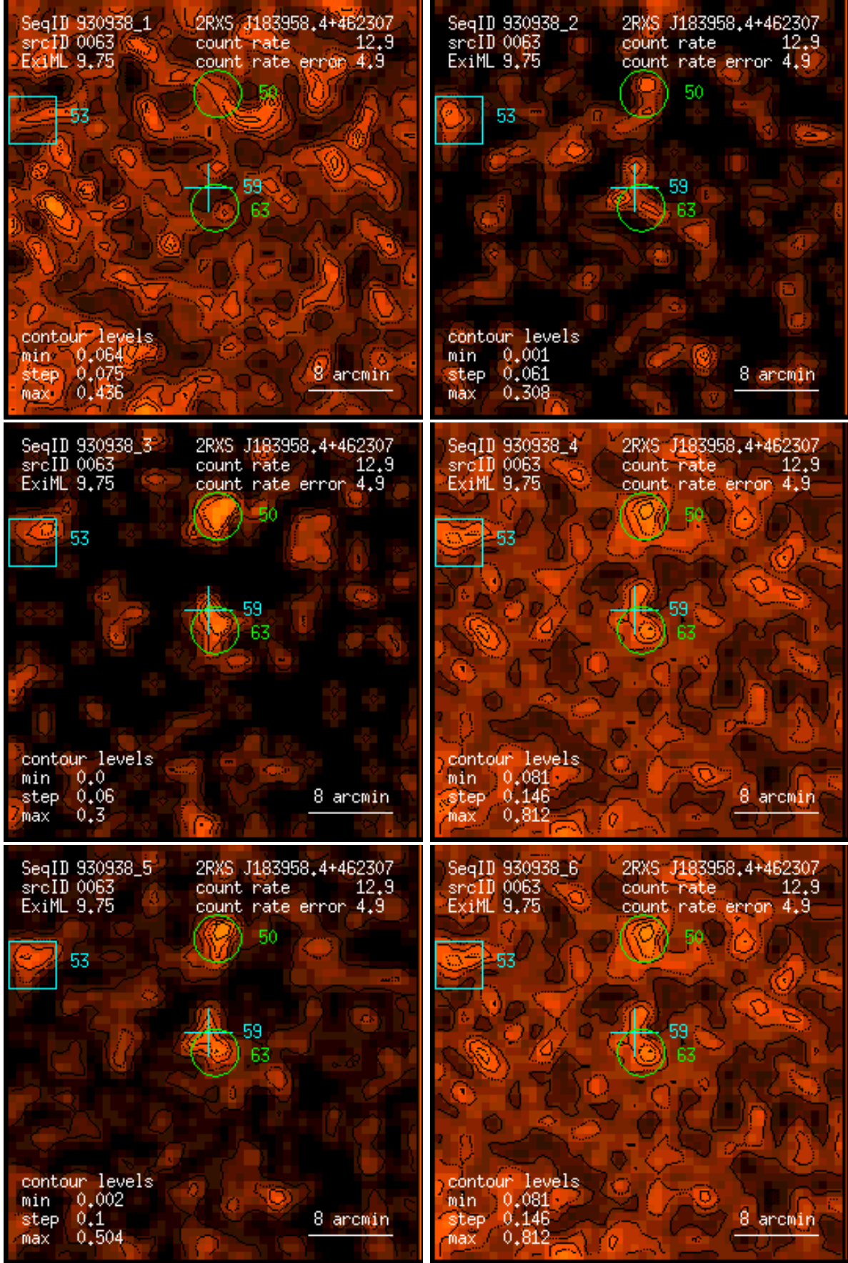
Figure 63: RASS 930938: detection 0063: band rate images, Gaussian filter: (1) PSPC channels 11 – 41, (2) 52 – 90, (3) 91 – 201, (4) 11 – 235, (5) 52 – 201, (6) 11 – 201. Broad band rates in counts/ks. Band rate contour levels in counts/ks/arcmin 2 .
