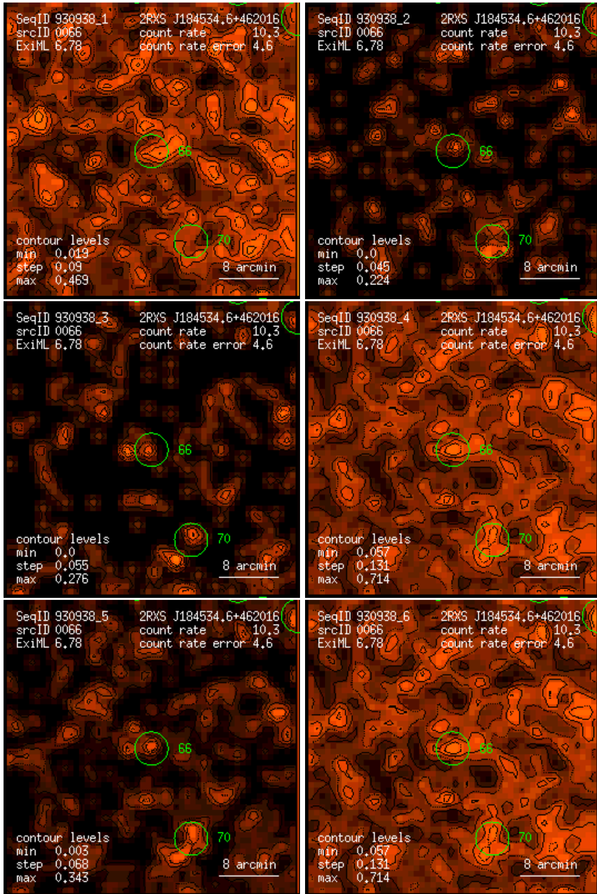
Figure 66: RASS 930938: detection 0066: band rate images, Gaussian filter: (1) PSPC channels 11 – 41, (2) 52 – 90, (3) 91 – 201, (4) 11 – 235, (5) 52 – 201, (6) 11 – 201. Broad band rates in counts/ks. Band rate contour levels in counts/ks/arcmin 2 .
