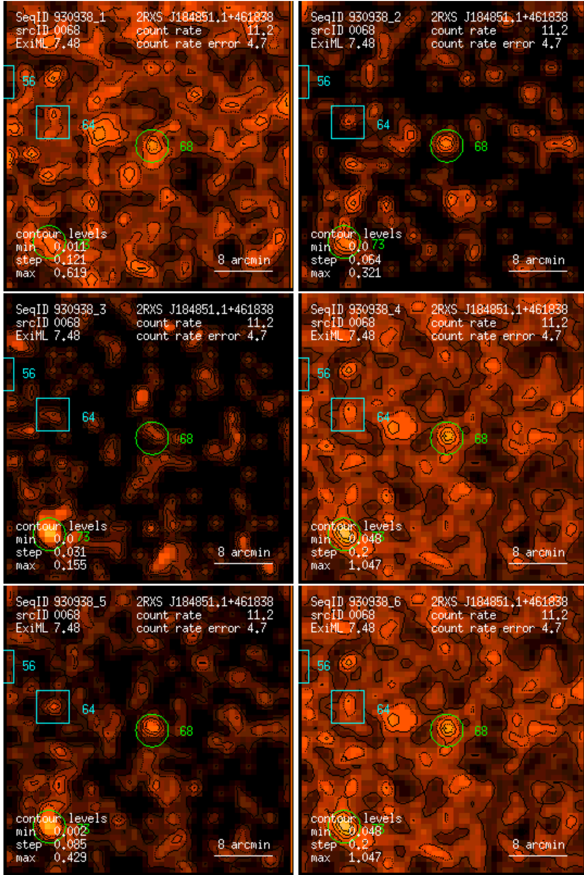
Figure 68: RASS 930938: detection 0068: band rate images, Gaussian filter: (1) PSPC channels 11 – 41, (2) 52 – 90, (3) 91 – 201, (4) 11 – 235, (5) 52 – 201, (6) 11 – 201. Broad band rates in counts/ks. Band rate contour levels in counts/ks/arcmin 2 .
