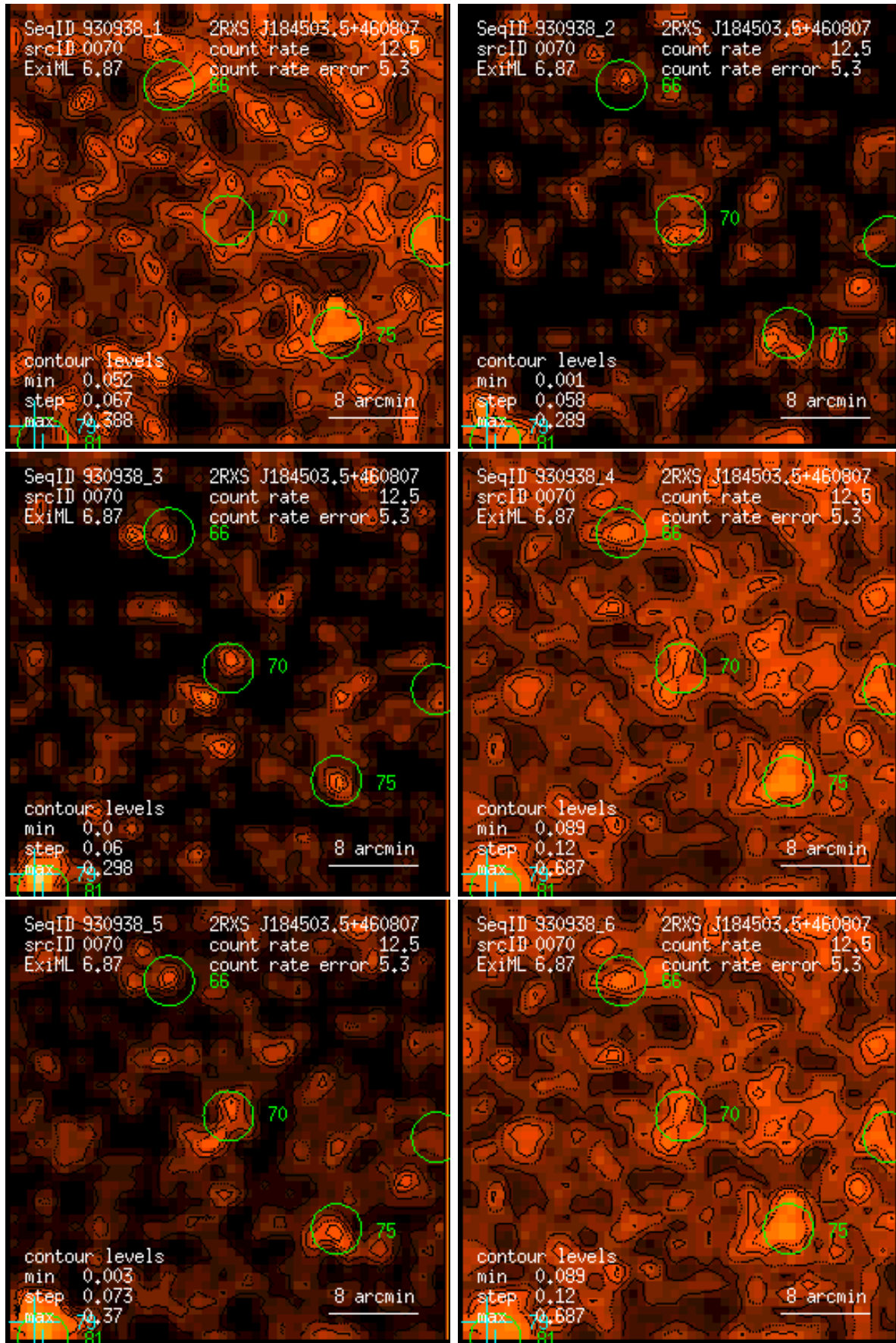
Figure 70: RASS 930938: detection 0070: band rate images, Gaussian filter: (1) PSPC channels 11 – 41, (2) 52 – 90, (3) 91 – 201, (4) 11 – 235, (5) 52 – 201, (6) 11 – 201. Broad band rates in counts/ks. Band rate contour levels in counts/ks/arcmin 2 .
