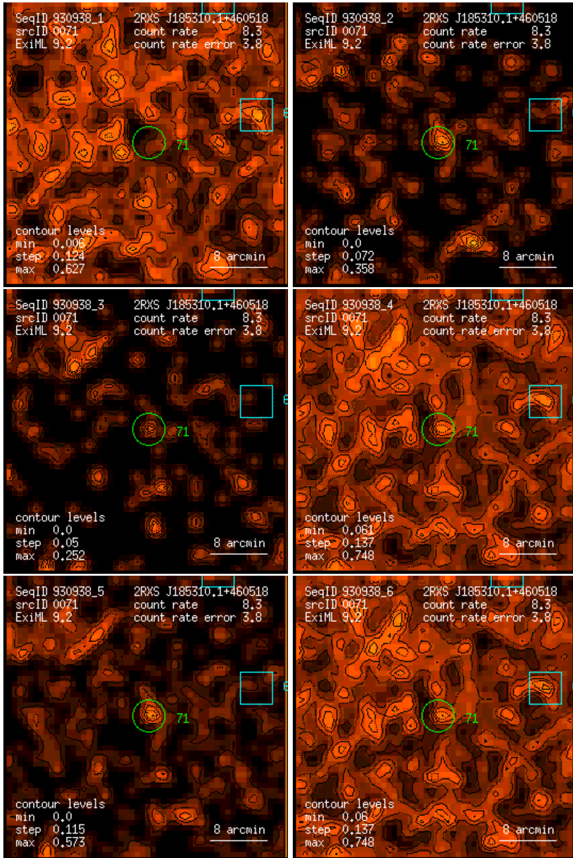
Figure 71: RASS 930938: detection 0071: band rate images, Gaussian filter: (1) PSPC channels 11 – 41, (2) 52 – 90, (3) 91 – 201, (4) 11 – 235, (5) 52 – 201, (6) 11 – 201. Broad band rates in counts/ks. Band rate contour levels in counts/ks/arcmin 2 .
