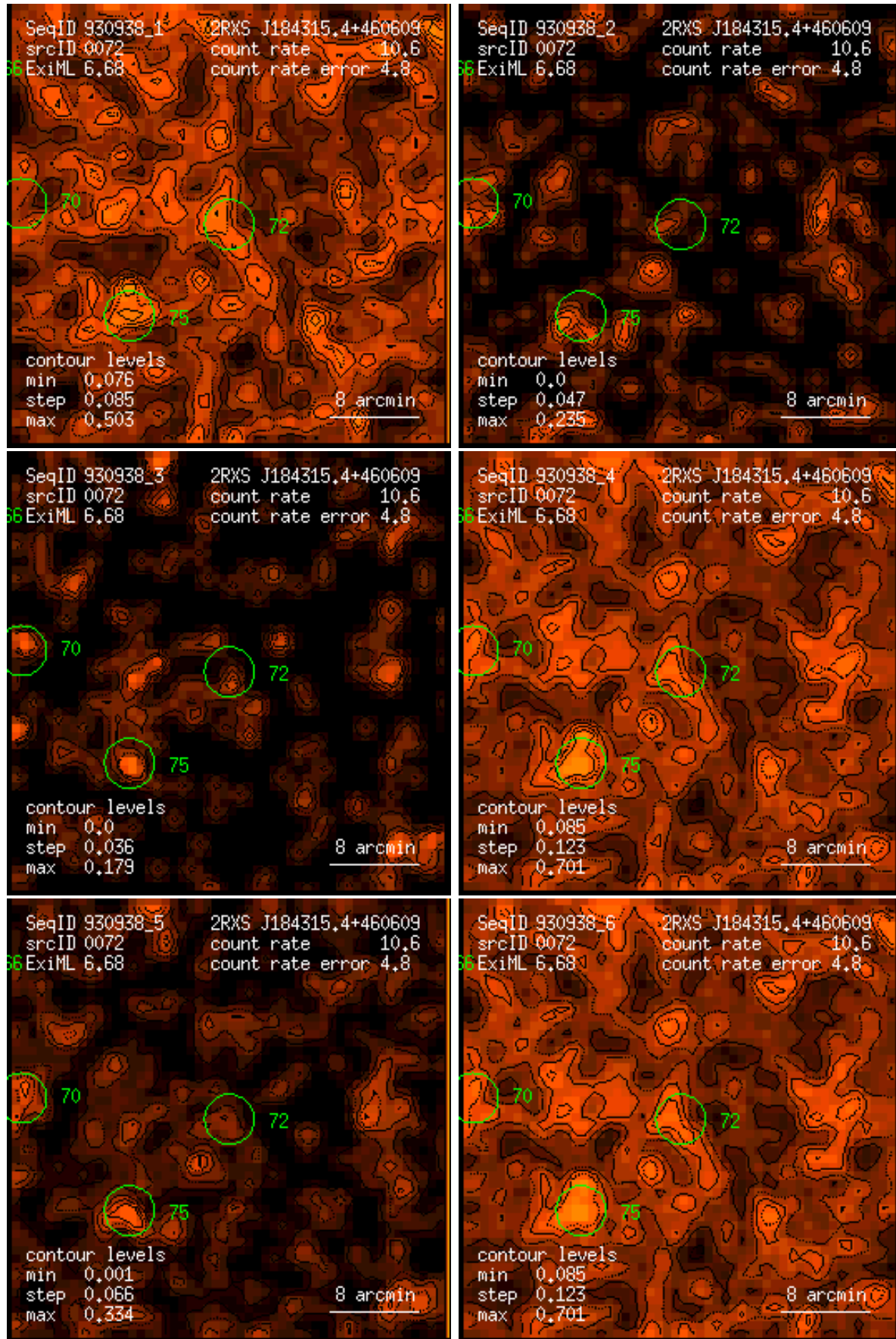
Figure 72: RASS 930938: detection 0072: band rate images, Gaussian filter: (1) PSPC channels 11 – 41, (2) 52 – 90, (3) 91 – 201, (4) 11 – 235, (5) 52 – 201, (6) 11 – 201. Broad band rates in counts/ks. Band rate contour levels in counts/ks/arcmin 2 .
