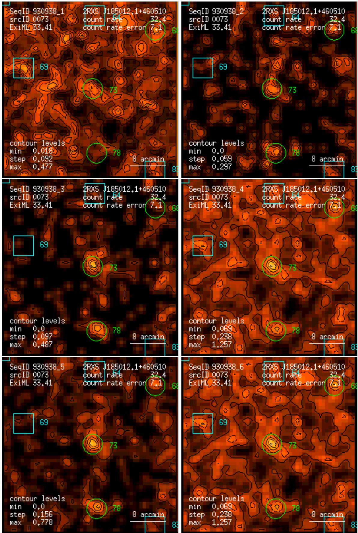
Figure 73: RASS 930938: detection 0073: band rate images, Gaussian filter: (1) PSPC channels 11 – 41, (2) 52 – 90, (3) 91 – 201, (4) 11 – 235, (5) 52 – 201, (6) 11 – 201. Broad band rates in counts/ks. Band rate contour levels in counts/ks/arcmin 2 .
