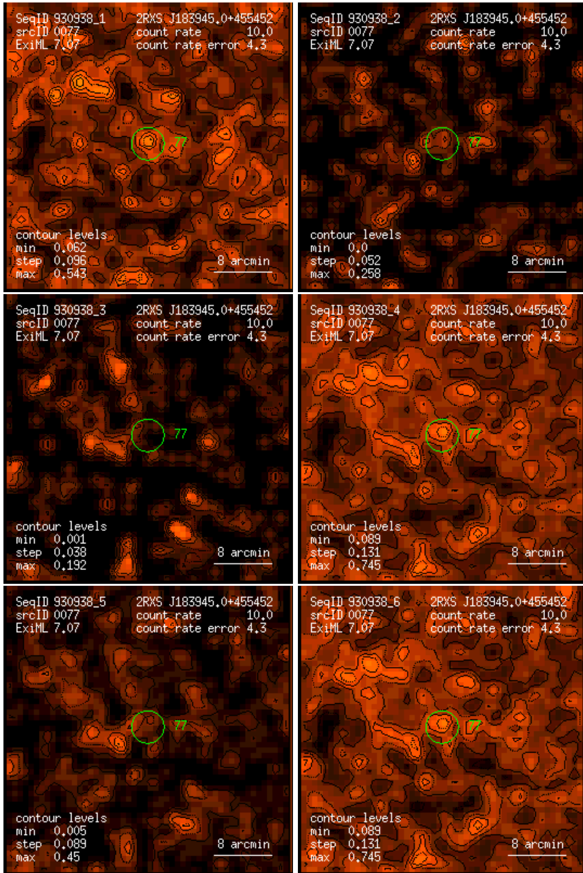
Figure 77: RASS 930938: detection 0077: band rate images, Gaussian filter: (1) PSPC channels 11 – 41, (2) 52 – 90, (3) 91 – 201, (4) 11 – 235, (5) 52 – 201, (6) 11 – 201. Broad band rates in counts/ks. Band rate contour levels in counts/ks/arcmin 2 .
