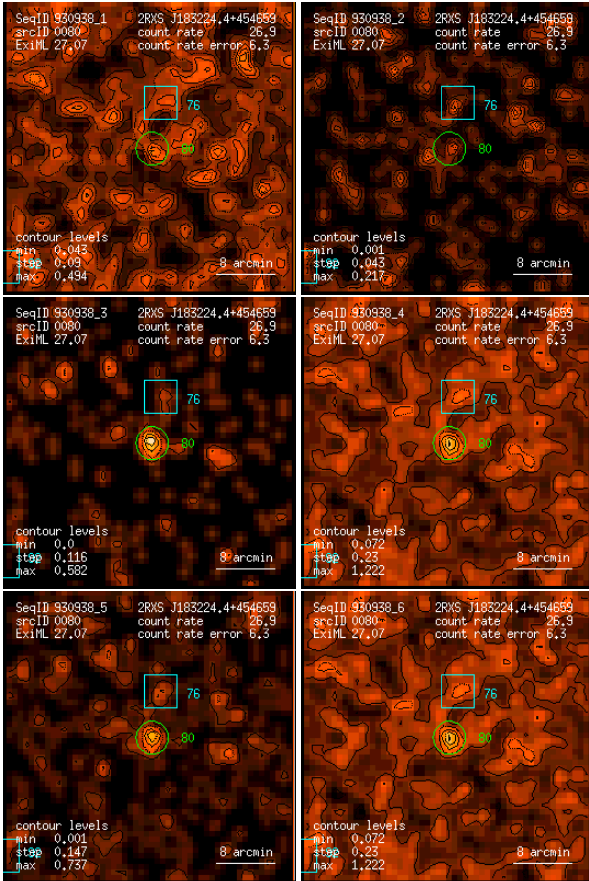
Figure 80: RASS 930938: detection 0080: band rate images, Gaussian filter: (1) PSPC channels 11 – 41, (2) 52 – 90, (3) 91 – 201, (4) 11 – 235, (5) 52 – 201, (6) 11 – 201. Broad band rates in counts/ks. Band rate contour levels in counts/ks/arcmin 2 .
