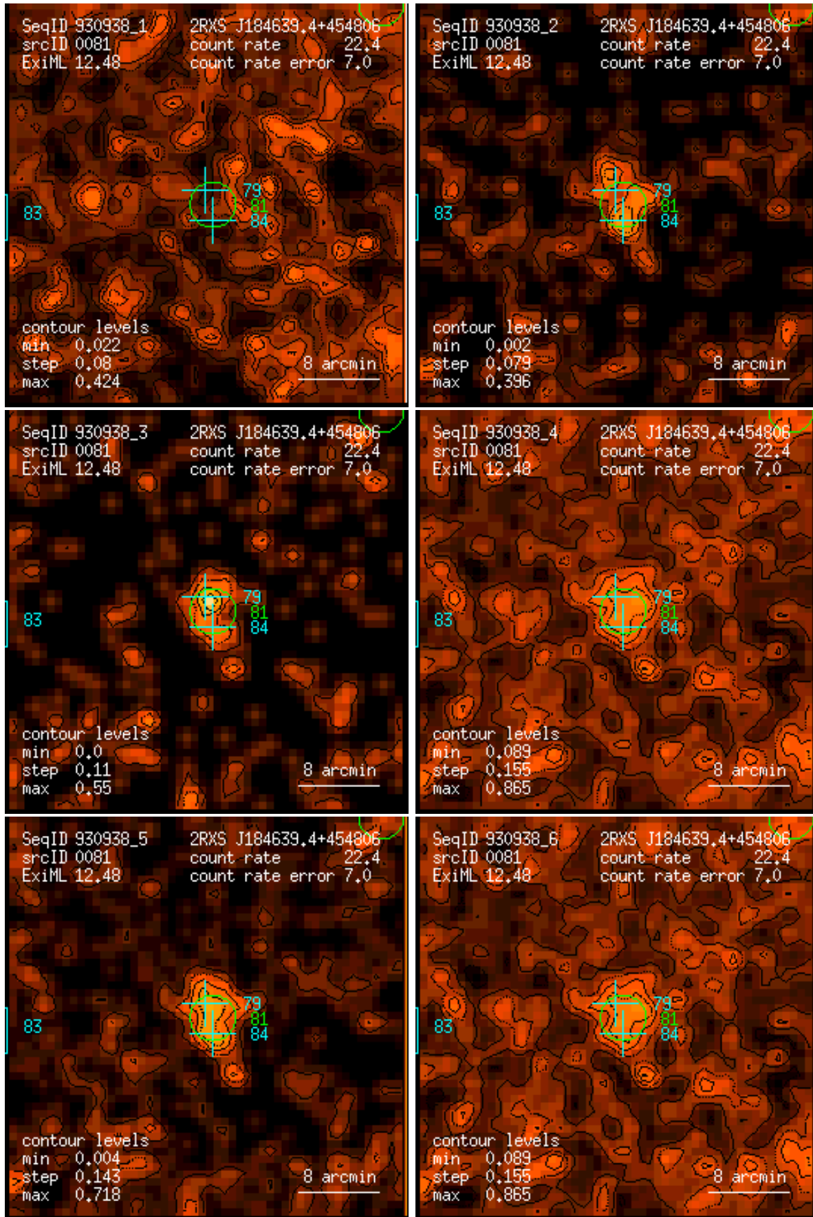
Figure 81: RASS 930938: detection 0081: band rate images, Gaussian filter: (1) PSPC channels 11 – 41, (2) 52 – 90, (3) 91 – 201, (4) 11 – 235, (5) 52 – 201, (6) 11 – 201. Broad band rates in counts/ks. Band rate contour levels in counts/ks/arcmin 2 .
