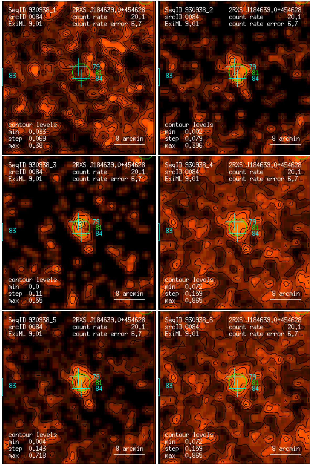
Figure 84: RASS 930938: detection 0084: band rate images, Gaussian filter: (1) PSPC channels 11 – 41, (2) 52 – 90, (3) 91 – 201, (4) 11 – 235, (5) 52 – 201, (6) 11 – 201. Broad band rates in counts/ks. Band rate contour levels in counts/ks/arcmin 2 .
