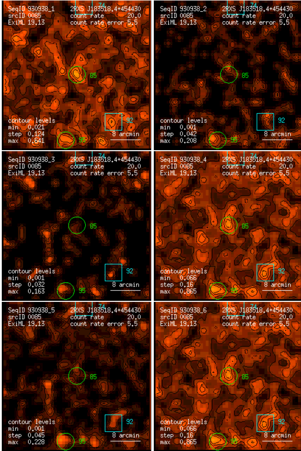
Figure 85: RASS 930938: detection 0085: band rate images, Gaussian filter: (1) PSPC channels 11 – 41, (2) 52 – 90, (3) 91 – 201, (4) 11 – 235, (5) 52 – 201, (6) 11 – 201. Broad band rates in counts/ks. Band rate contour levels in counts/ks/arcmin 2 .
