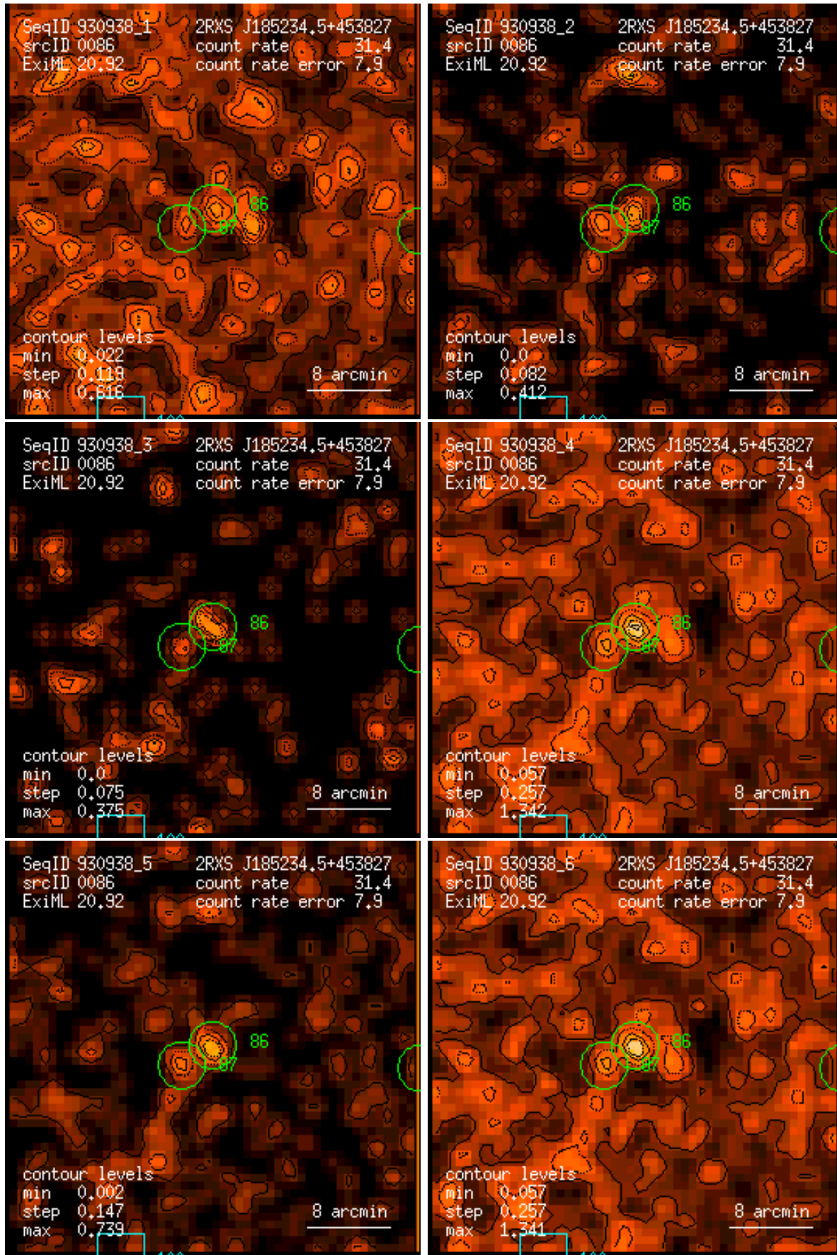
Figure 86: RASS 930938: detection 0086: band rate images, Gaussian filter: (1) PSPC channels 11 – 41, (2) 52 – 90, (3) 91 – 201, (4) 11 – 235, (5) 52 – 201, (6) 11 – 201. Broad band rates in counts/ks. Band rate contour levels in counts/ks/arcmin 2 .
