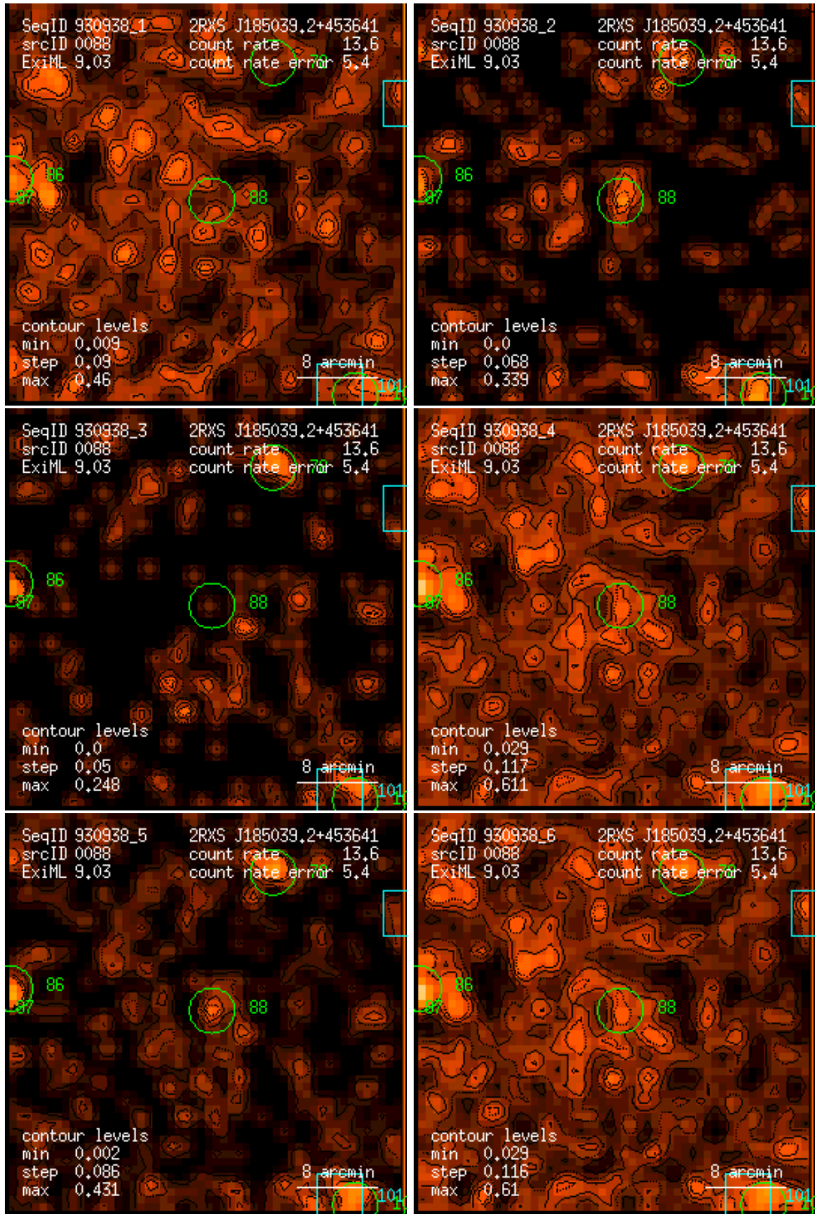
Figure 88: RASS 930938: detection 0088: band rate images, Gaussian filter: (1) PSPC channels 11 – 41, (2) 52 – 90, (3) 91 – 201, (4) 11 – 235, (5) 52 – 201, (6) 11 – 201. Broad band rates in counts/ks. Band rate contour levels in counts/ks/arcmin 2 .
