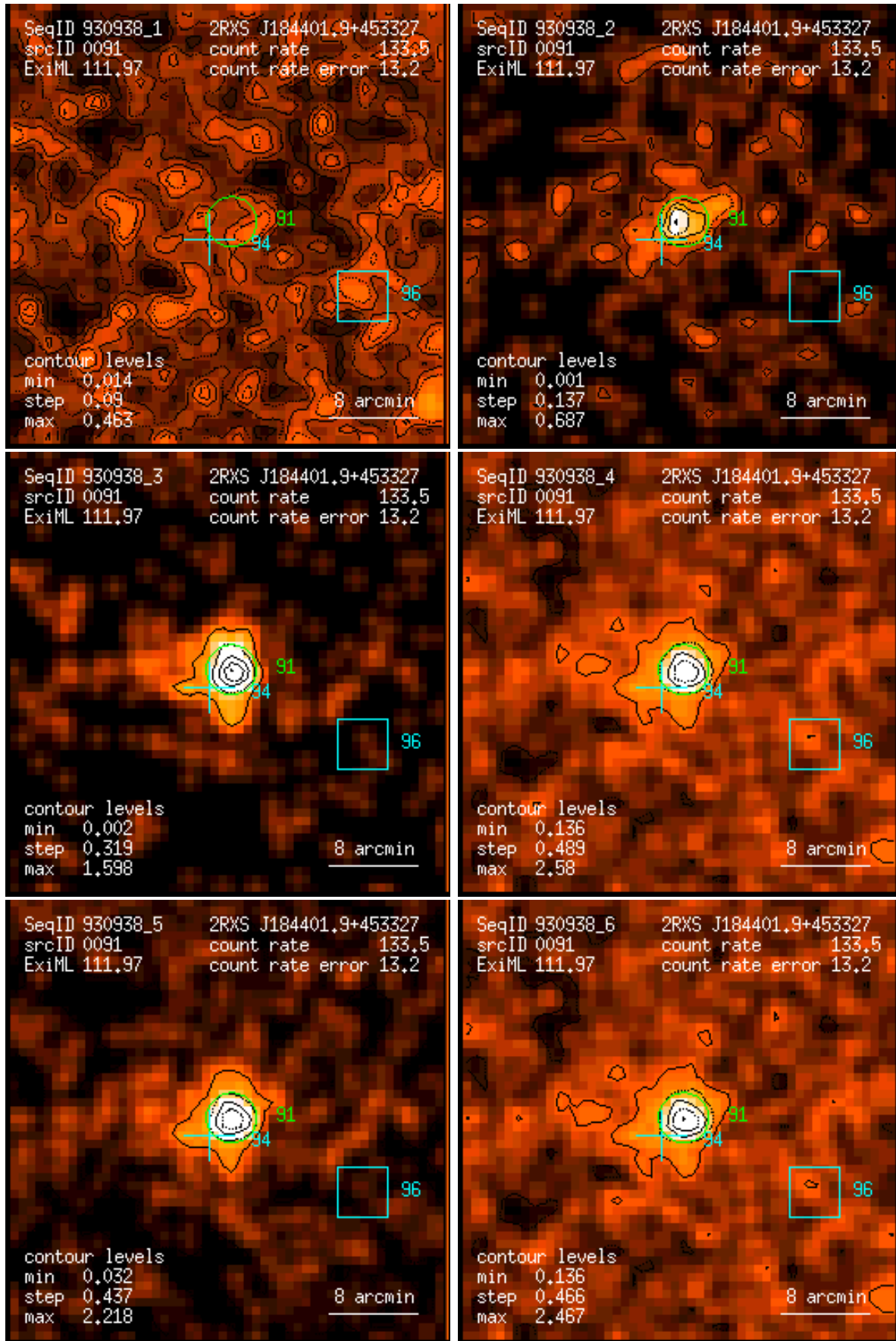
Figure 91: RASS 930938: detection 0091: band rate images, Gaussian filter: (1) PSPC channels 11 – 41, (2) 52 – 90, (3) 91 – 201, (4) 11 – 235, (5) 52 – 201, (6) 11 – 201. Broad band rates in counts/ks. Band rate contour levels in counts/ks/arcmin 2 .
