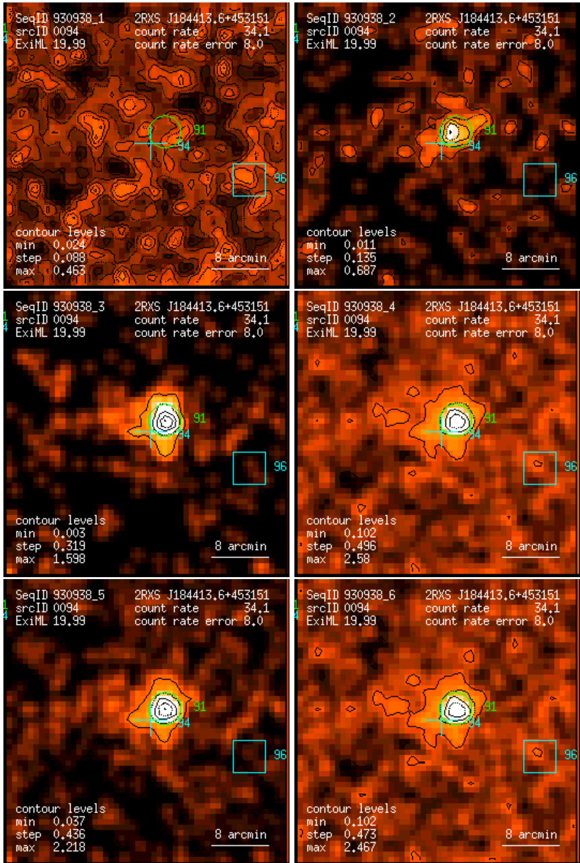
Figure 94: RASS 930938: detection 0094: band rate images, Gaussian filter: (1) PSPC channels 11 – 41, (2) 52 – 90, (3) 91 – 201, (4) 11 – 235, (5) 52 – 201, (6) 11 – 201. Broad band rates in counts/ks. Band rate contour levels in counts/ks/arcmin 2 .
