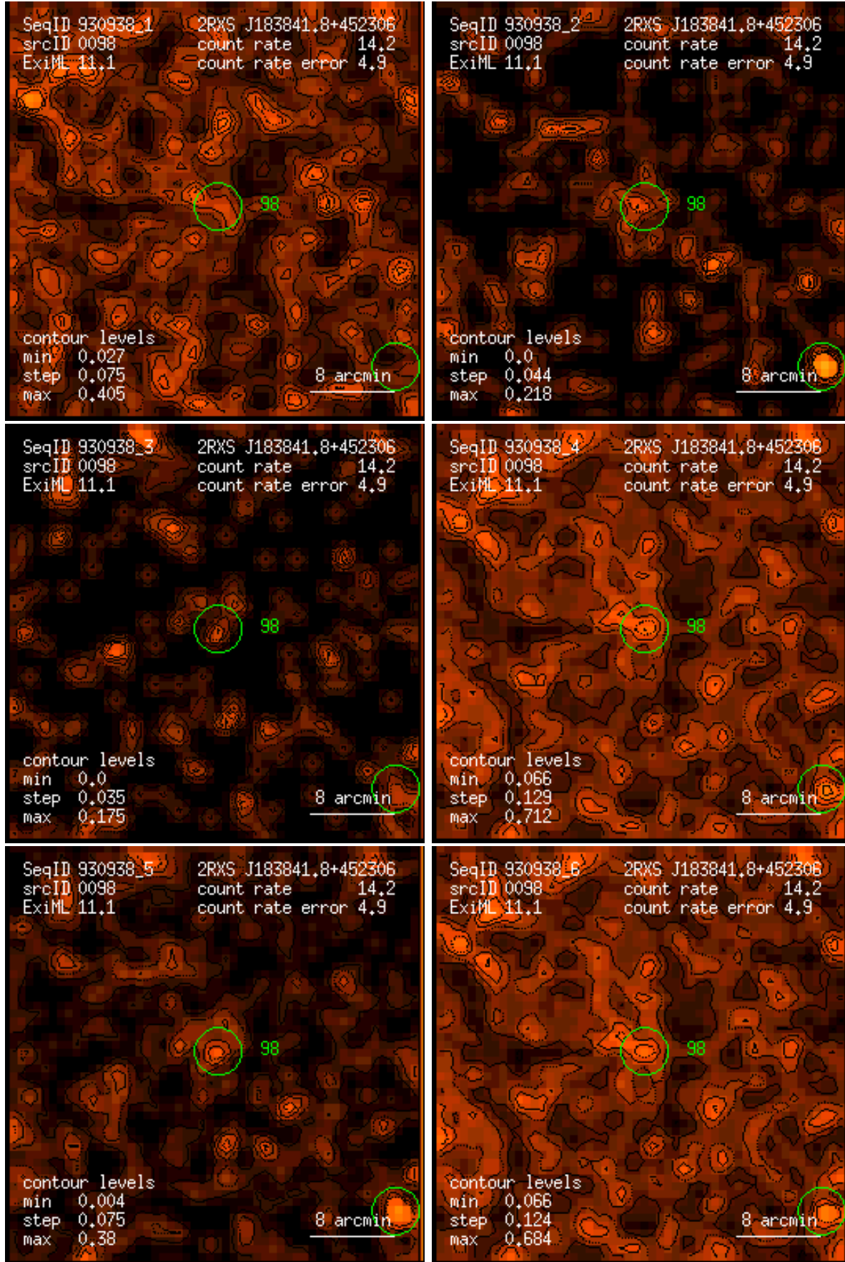
Figure 98: RASS 930938: detection 0098: band rate images, Gaussian filter: (1) PSPC channels 11 – 41, (2) 52 – 90, (3) 91 – 201, (4) 11 – 235, (5) 52 – 201, (6) 11 – 201. Broad band rates in counts/ks. Band rate contour levels in counts/ks/arcmin 2 .
