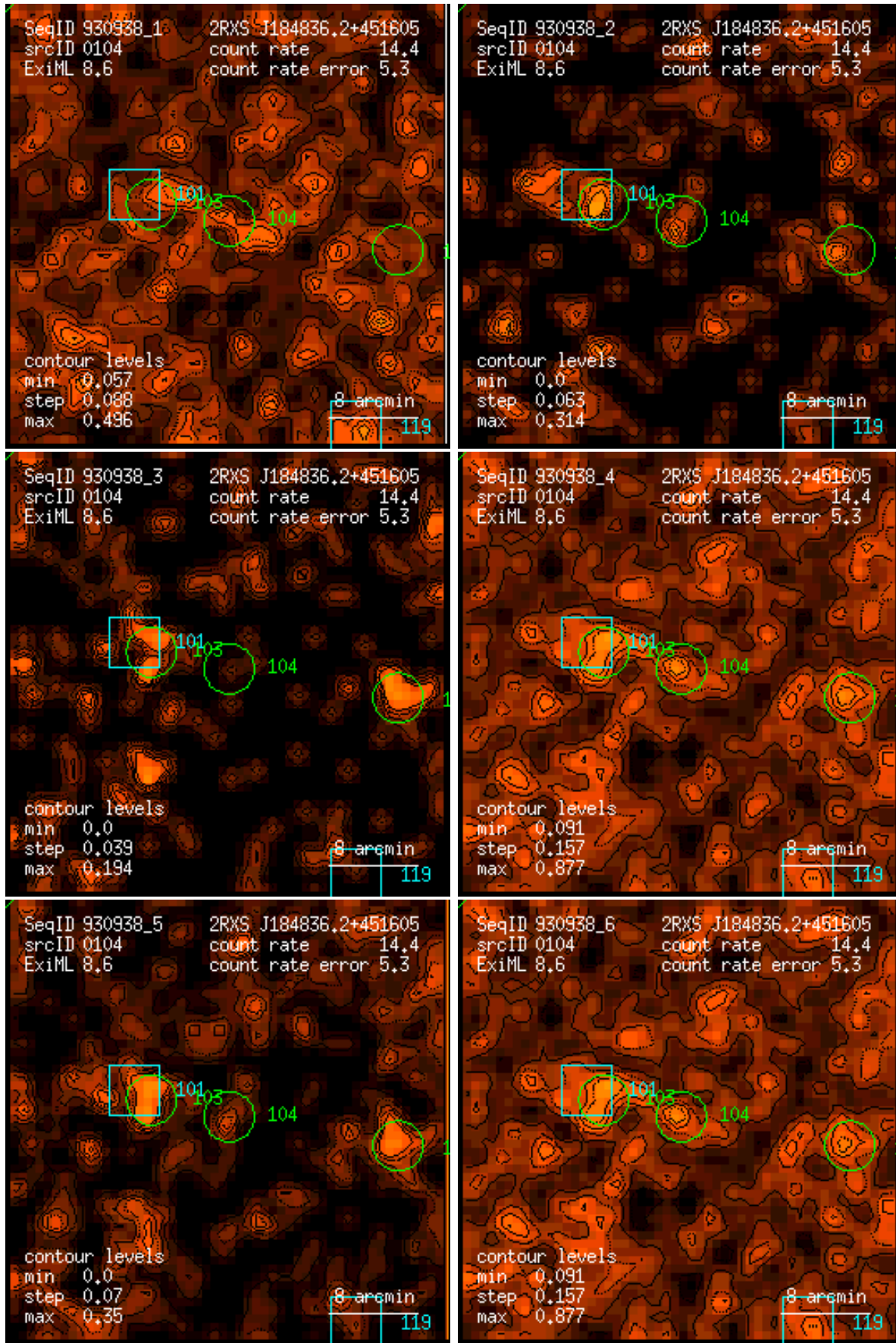
Figure 104: RASS 930938: detection 0104: band rate images, Gaussian filter: (1) PSPC channels 11 – 41, (2) 52 – 90, (3) 91 – 201, (4) 11 – 235, (5) 52 – 201, (6) 11 – 201. Broad band rates in counts/ks. Band rate contour levels in counts/ks/arcmin 2 .
