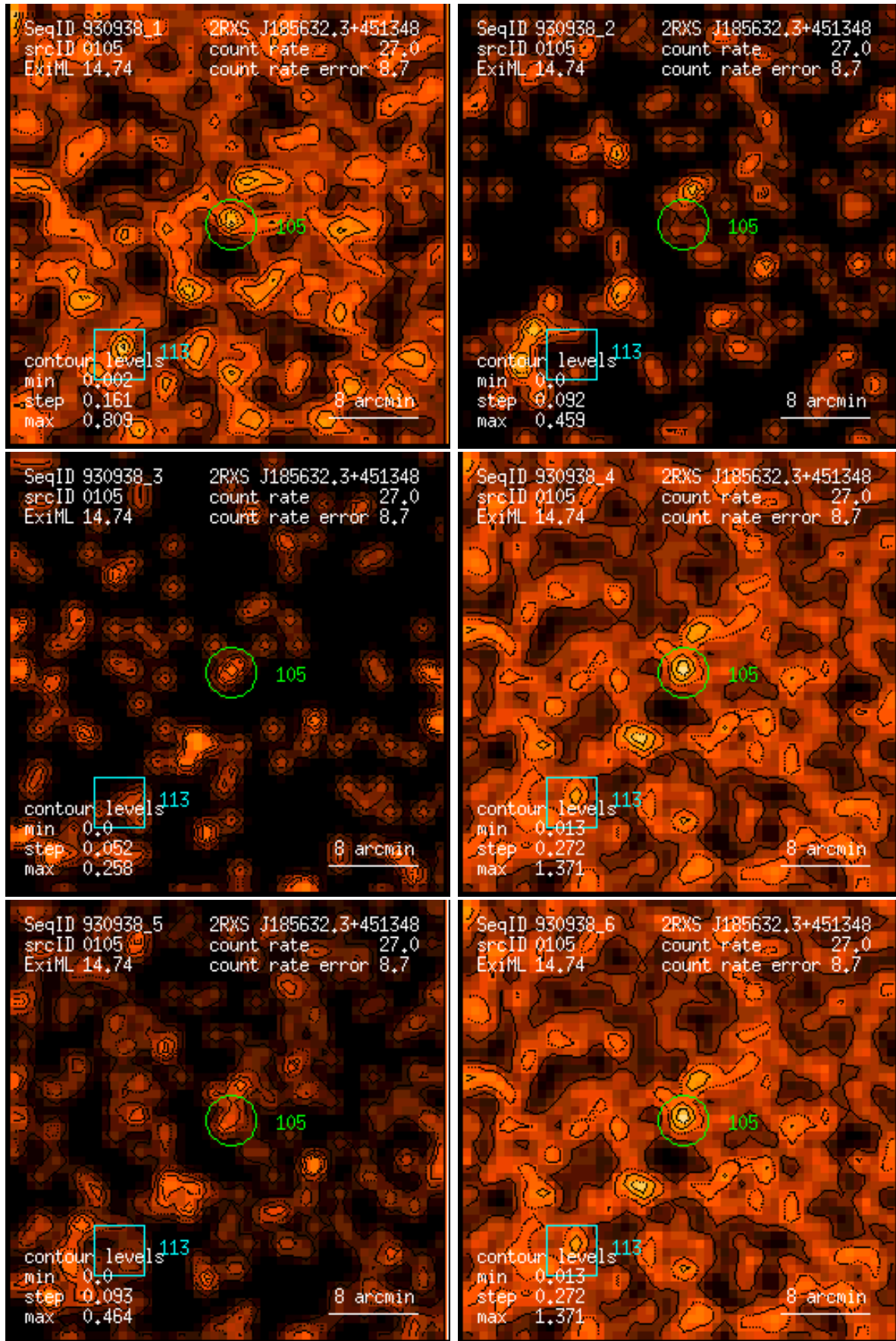
Figure 105: RASS 930938: detection 0105: band rate images, Gaussian filter: (1) PSPC channels 11 – 41, (2) 52 – 90, (3) 91 – 201, (4) 11 – 235, (5) 52 – 201, (6) 11 – 201. Broad band rates in counts/ks. Band rate contour levels in counts/ks/arcmin 2 .
