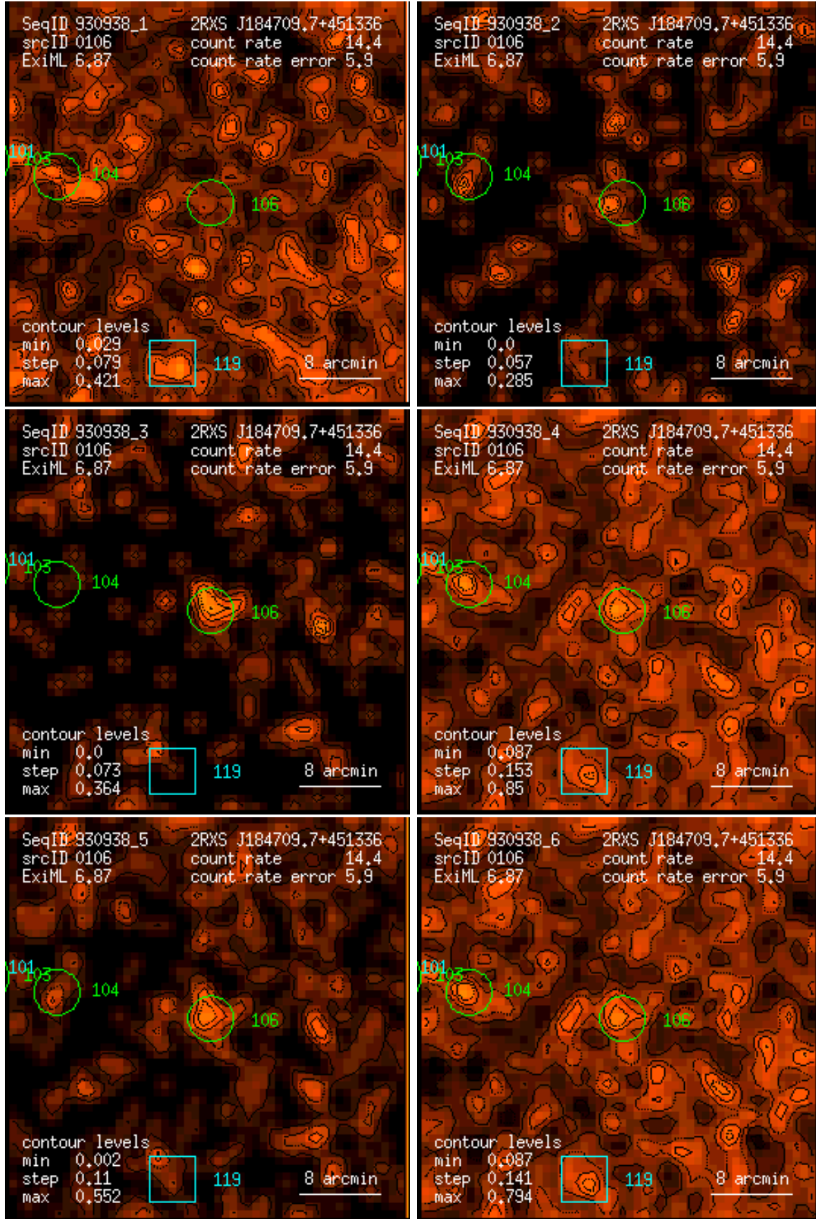
Figure 106: RASS 930938: detection 0106: band rate images, Gaussian filter: (1) PSPC channels 11 – 41, (2) 52 – 90, (3) 91 – 201, (4) 11 – 235, (5) 52 – 201, (6) 11 – 201. Broad band rates in counts/ks. Band rate contour levels in counts/ks/arcmin 2 .
