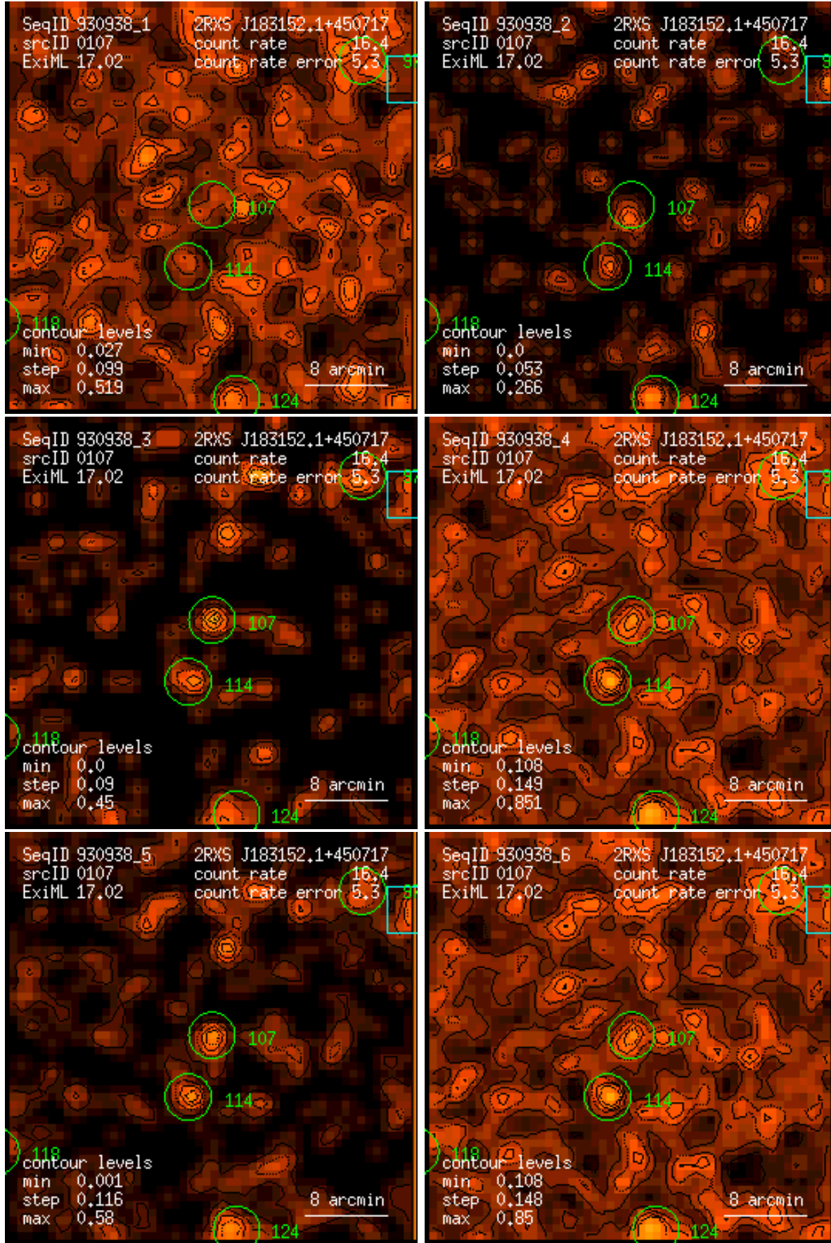
Figure 107: RASS 930938: detection 0107: band rate images, Gaussian filter: (1) PSPC channels 11 – 41, (2) 52 – 90, (3) 91 – 201, (4) 11 – 235, (5) 52 – 201, (6) 11 – 201. Broad band rates in counts/ks. Band rate contour levels in counts/ks/arcmin 2 .
