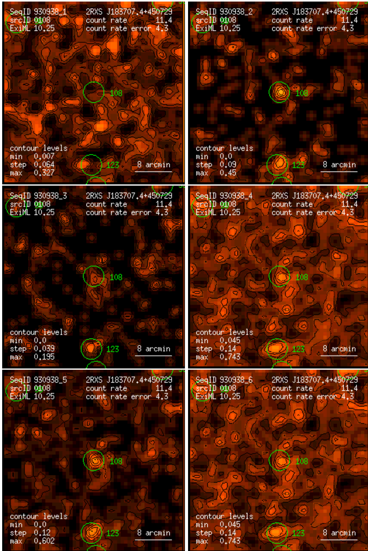
Figure 108: RASS 930938: detection 0108: band rate images, Gaussian filter: (1) PSPC channels 11 – 41, (2) 52 – 90, (3) 91 – 201, (4) 11 – 235, (5) 52 – 201, (6) 11 – 201. Broad band rates in counts/ks. Band rate contour levels in counts/ks/arcmin 2 .
