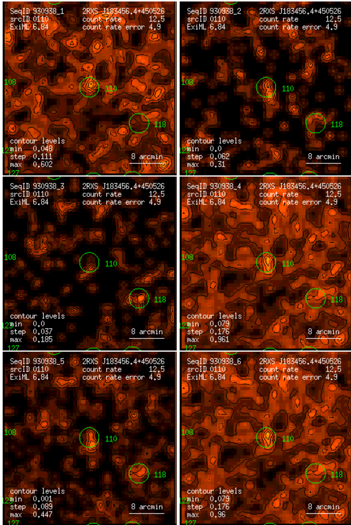
Figure 110: RASS 930938: detection 0110: band rate images, Gaussian filter: (1) PSPC channels 11 – 41, (2) 52 – 90, (3) 91 – 201, (4) 11 – 235, (5) 52 – 201, (6) 11 – 201. Broad band rates in counts/ks. Band rate contour levels in counts/ks/arcmin 2 .
