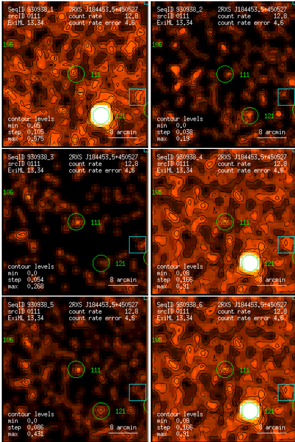
Figure 111: RASS 930938: detection 0111: band rate images, Gaussian filter: (1) PSPC channels 11 – 41, (2) 52 – 90, (3) 91 – 201, (4) 11 – 235, (5) 52 – 201, (6) 11 – 201. Broad band rates in counts/ks. Band rate contour levels in counts/ks/arcmin 2 .
