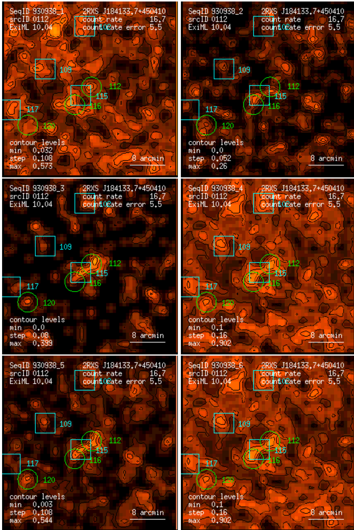
Figure 112: RASS 930938: detection 0112: band rate images, Gaussian filter: (1) PSPC channels 11 – 41, (2) 52 – 90, (3) 91 – 201, (4) 11 – 235, (5) 52 – 201, (6) 11 – 201. Broad band rates in counts/ks. Band rate contour levels in counts/ks/arcmin 2 .
