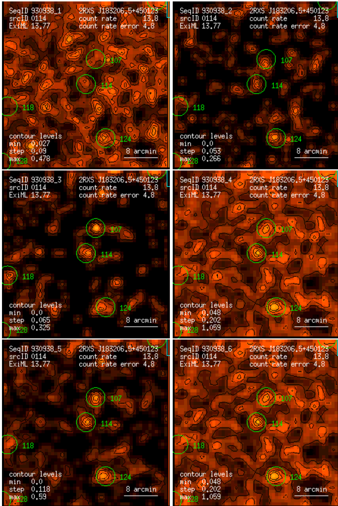
Figure 114: RASS 930938: detection 0114: band rate images, Gaussian filter: (1) PSPC channels 11 – 41, (2) 52 – 90, (3) 91 – 201, (4) 11 – 235, (5) 52 – 201, (6) 11 – 201. Broad band rates in counts/ks. Band rate contour levels in counts/ks/arcmin 2 .
