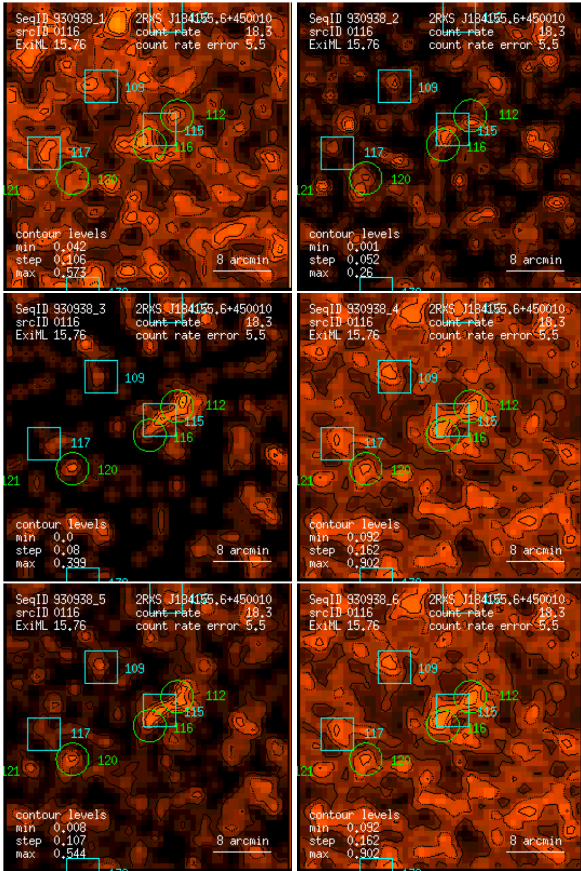
Figure 116: RASS 930938: detection 0116: band rate images, Gaussian filter: (1) PSPC channels 11 – 41, (2) 52 – 90, (3) 91 – 201, (4) 11 – 235, (5) 52 – 201, (6) 11 – 201. Broad band rates in counts/ks. Band rate contour levels in counts/ks/arcmin 2 .
