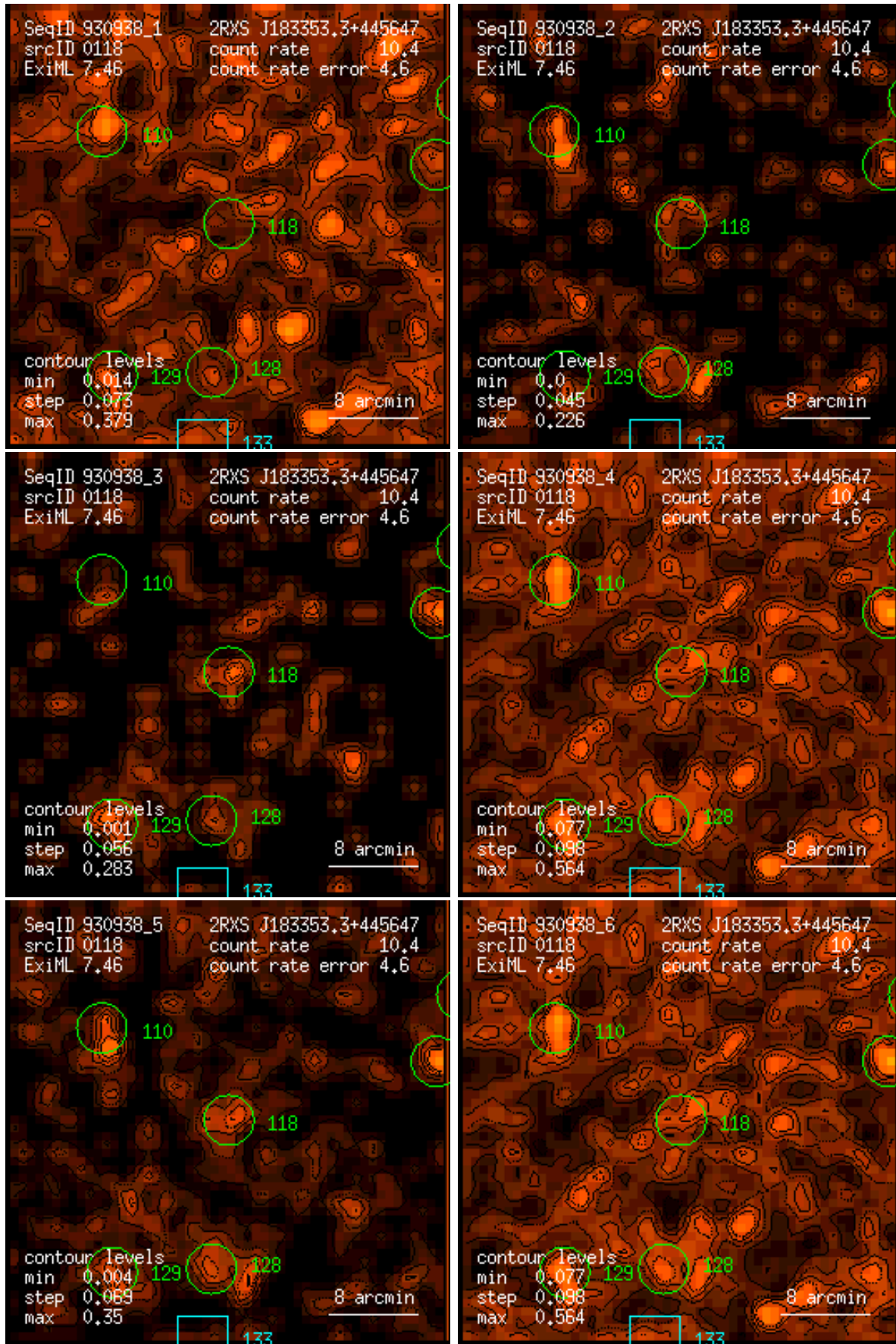
Figure 118: RASS 930938: detection 0118: band rate images, Gaussian filter: (1) PSPC channels 11 – 41, (2) 52 – 90, (3) 91 – 201, (4) 11 – 235, (5) 52 – 201, (6) 11 – 201. Broad band rates in counts/ks. Band rate contour levels in counts/ks/arcmin 2 .
