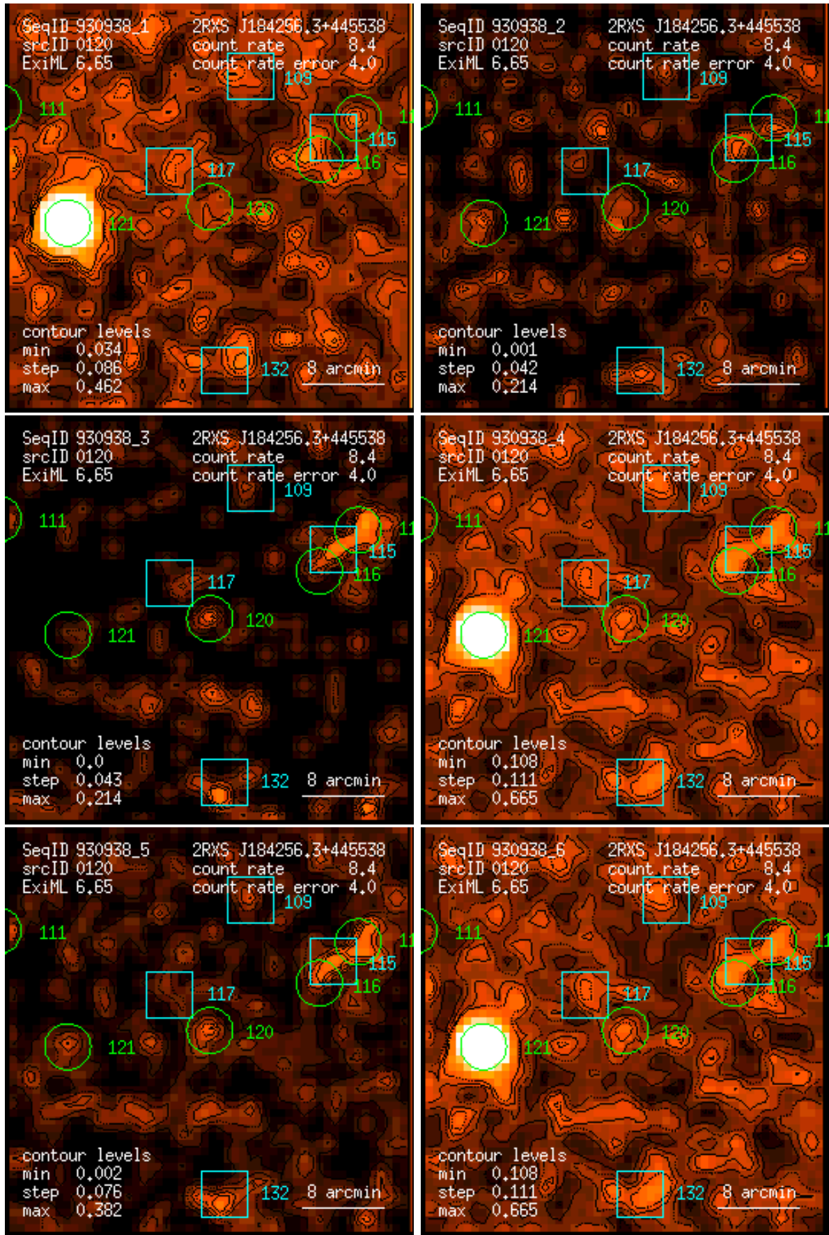
Figure 120: RASS 930938: detection 0120: band rate images, Gaussian filter: (1) PSPC channels 11 – 41, (2) 52 – 90, (3) 91 – 201, (4) 11 – 235, (5) 52 – 201, (6) 11 – 201. Broad band rates in counts/ks. Band rate contour levels in counts/ks/arcmin 2 .
