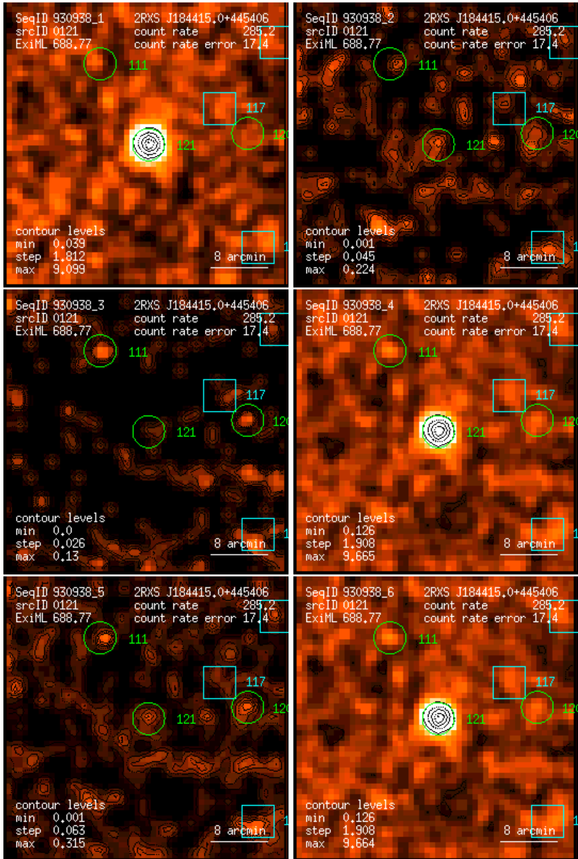
Figure 121: RASS 930938: detection 0121: band rate images, Gaussian filter: (1) PSPC channels 11 – 41, (2) 52 – 90, (3) 91 – 201, (4) 11 – 235, (5) 52 – 201, (6) 11 – 201. Broad band rates in counts/ks. Band rate contour levels in counts/ks/arcmin 2 .
