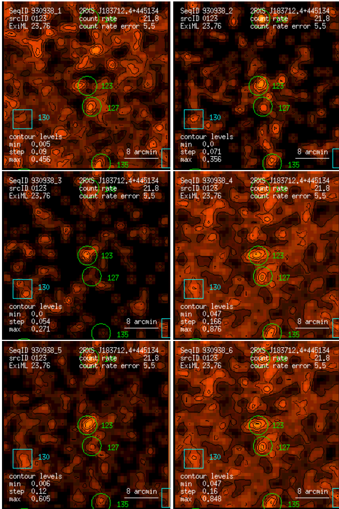
Figure 123: RASS 930938: detection 0123: band rate images, Gaussian filter: (1) PSPC channels 11 – 41, (2) 52 – 90, (3) 91 – 201, (4) 11 – 235, (5) 52 – 201, (6) 11 – 201. Broad band rates in counts/ks. Band rate contour levels in counts/ks/arcmin 2 .
